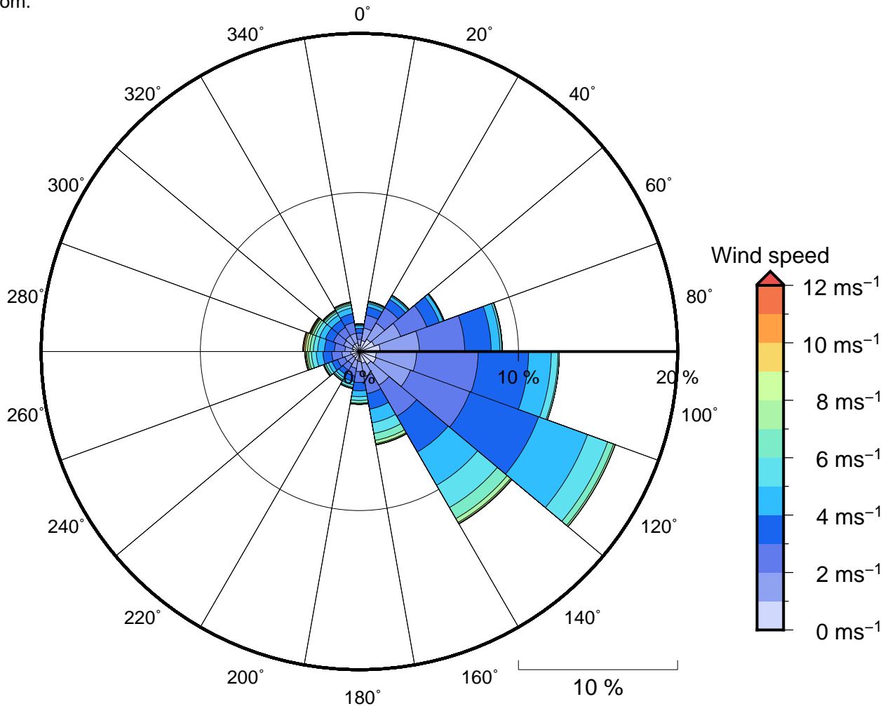
Figure 11 Annual wind rose for Ghizo. Note that directions are where the wind is coming from .
