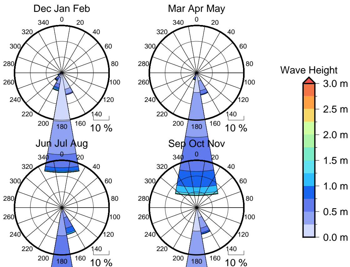
Figure 3 Seasonal wave roses for Ghizo
