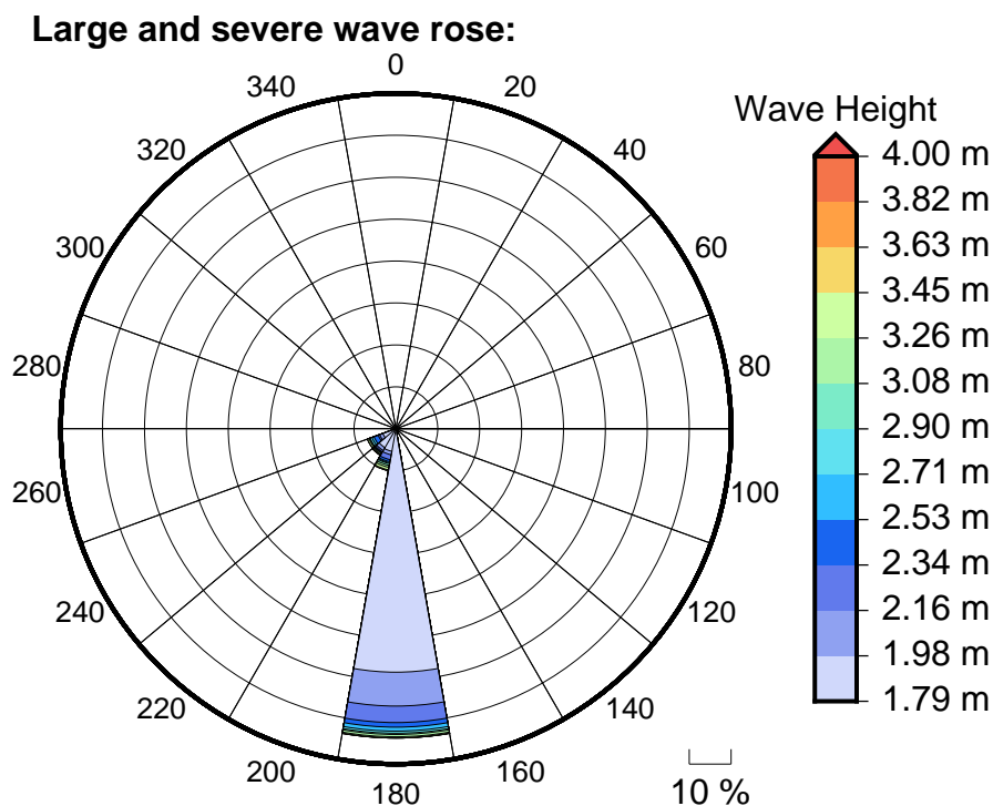
Figure 6 Large, severe and extreme wave roses for Ghizo
