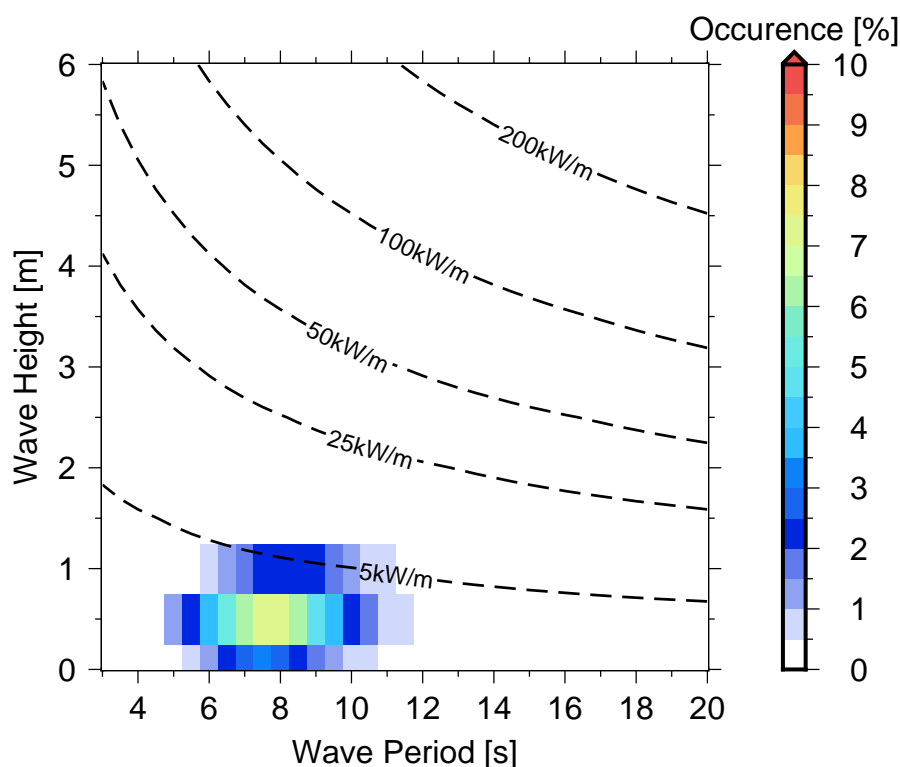
Figure 10 Occurrences of sea states in Ghizo .
