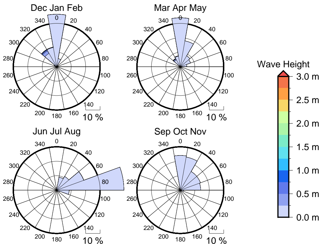
Figure 3 Seasonal wave roses for Honiara
