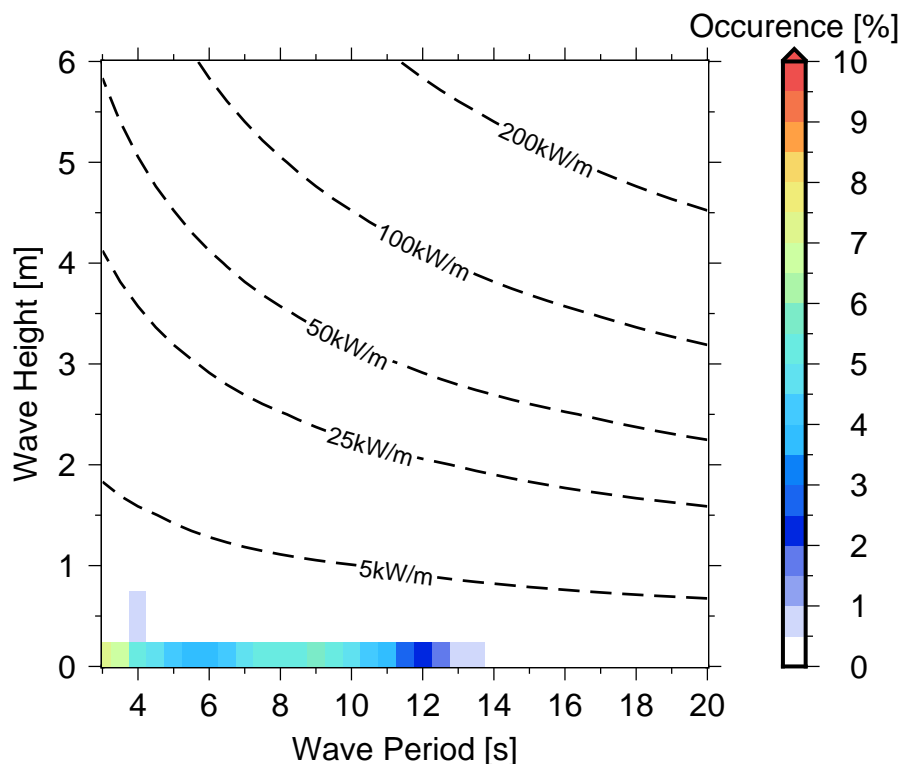
Figure 10 Occurrences of sea states in Honiara .
