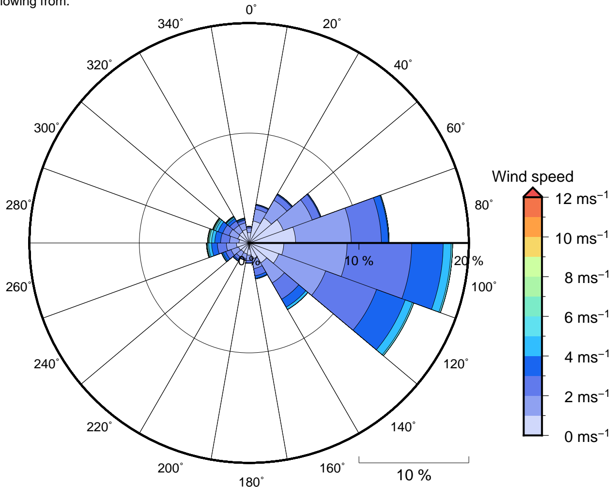
Figure 11 Annual wind rose for Honiara. Note that directions are where the wind is coming from.
