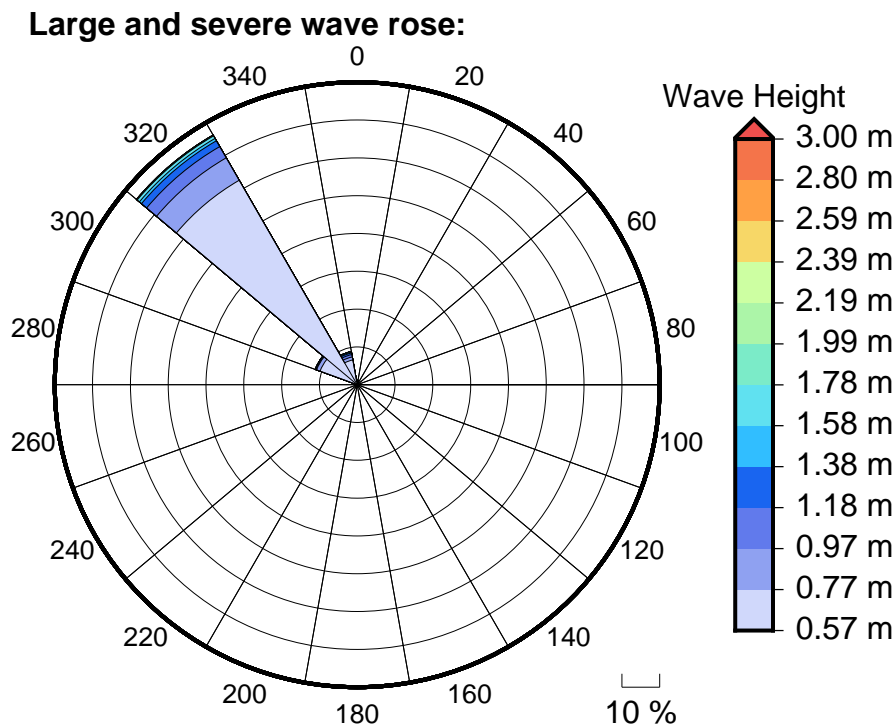
Figure 6 Large, severe and extreme wave roses for Honiara
