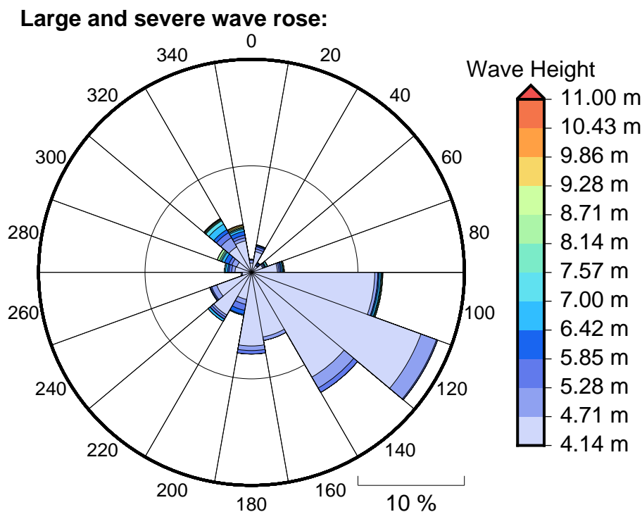
Figure 6 Large, severe and extreme wave roses for 'Eua Wave Buoy
