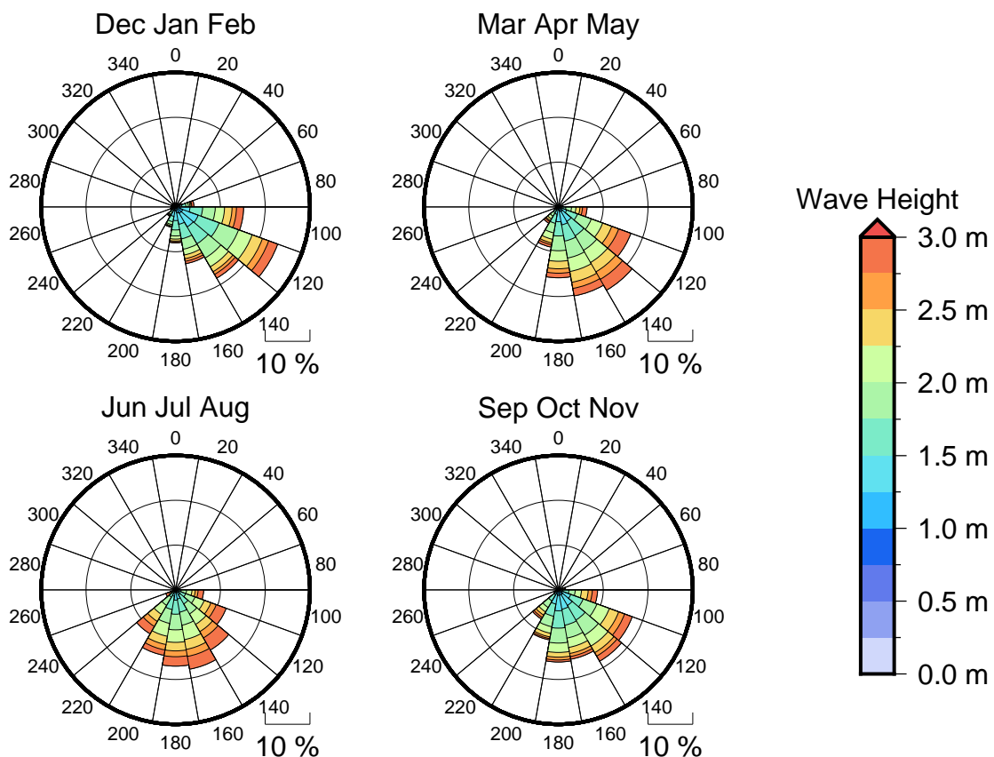
Figure 3 Seasonal wave roses for 'Eua Wave Buoy
