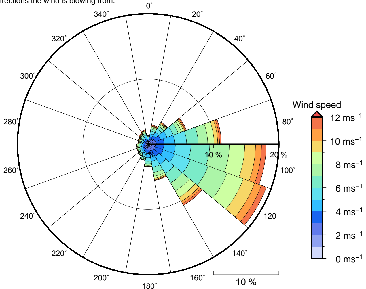
Figure 11 Annual wind rose for 'Eua Wave Buoy. Note that directions are where the wind is coming from.
