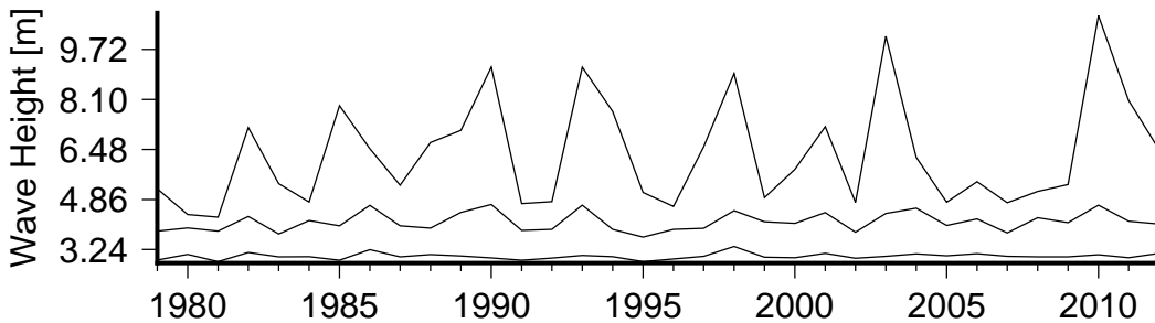
Figure 8 Annual variation in large waves (90th percentile)(lower curve), severe waves (99th percentile) (middle curve) and the largest wave(upper curve) in 'Eua Wave Buoy.
