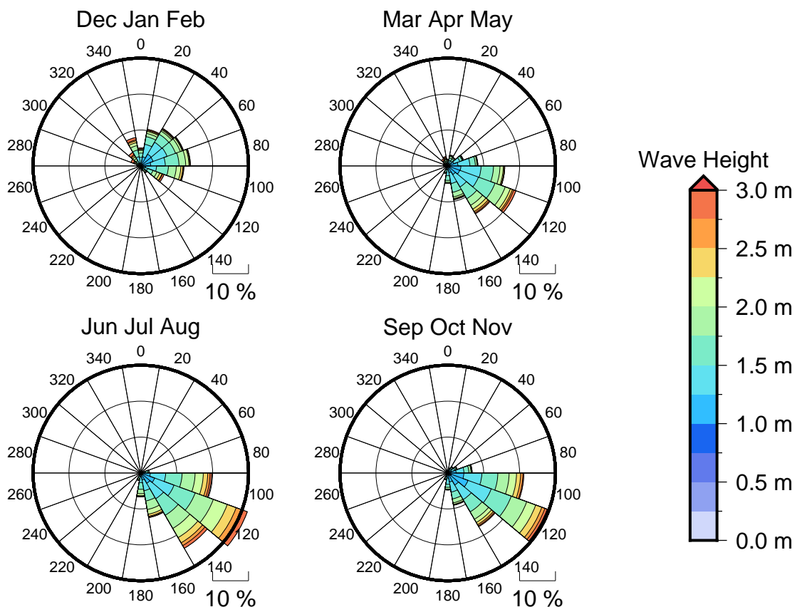
Figure 3 Seasonal wave roses for Niua
