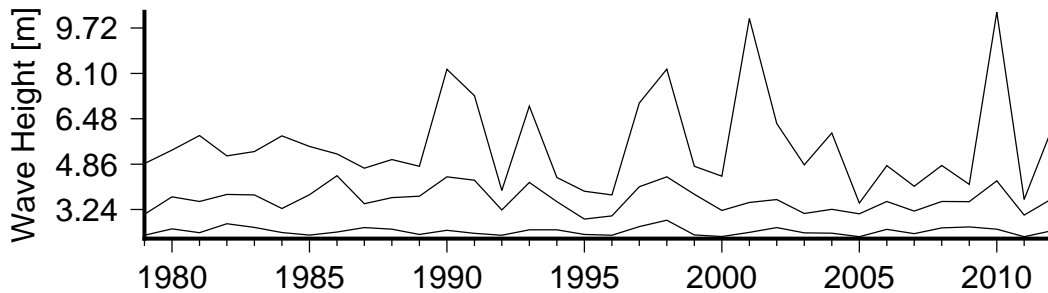
Figure 8 Annual variation in large waves (90th percentile)(lower curve), severe waves (99th percentile) (middle curve) and the largest wave(upper curve) in Niuaus.
