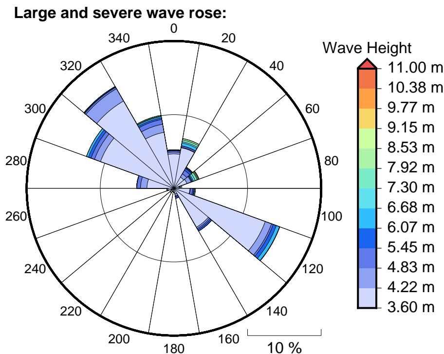
Figure 6 Large, severe and extreme wave roses for Niuaus
