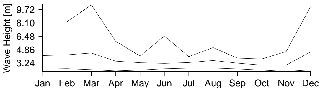
Figure 7 Monthly variation in large waves (90th percentile)(lower curve), severe waves (99th percentile) (middle curve) and the largest wave(upper curve) in Niuaus.
