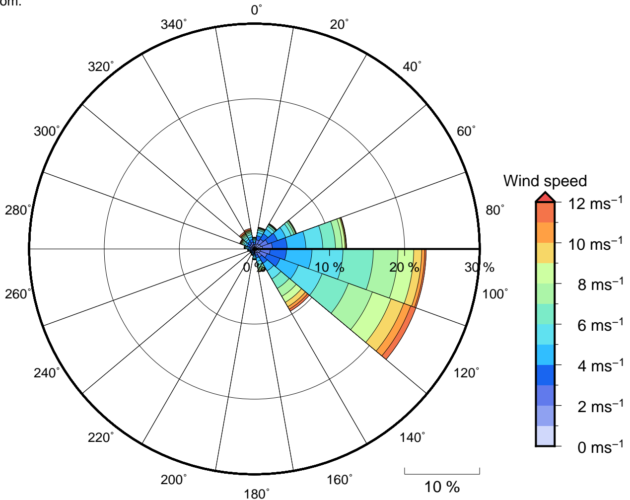
Figure 11 Annual wind rose for Niuas. Note that directions are where the wind is coming from.
