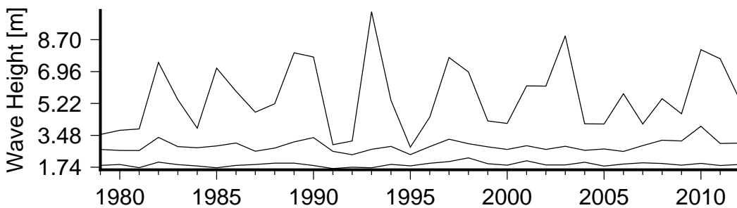
Figure 8 Annual variation in large waves (90th percentile)(lower curve), severe waves (99th percentile) (middle curve) and the largest wave(upper curve) in Nuku'alofa.
