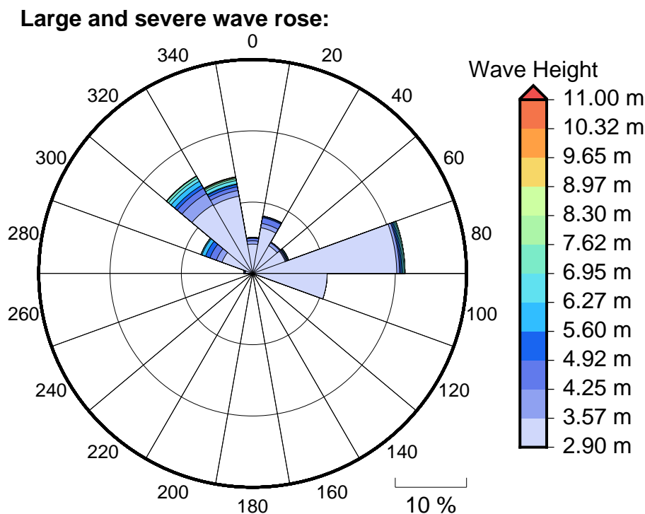
Figure 6 Large, severe and extreme wave roses for Nuku'alofa
