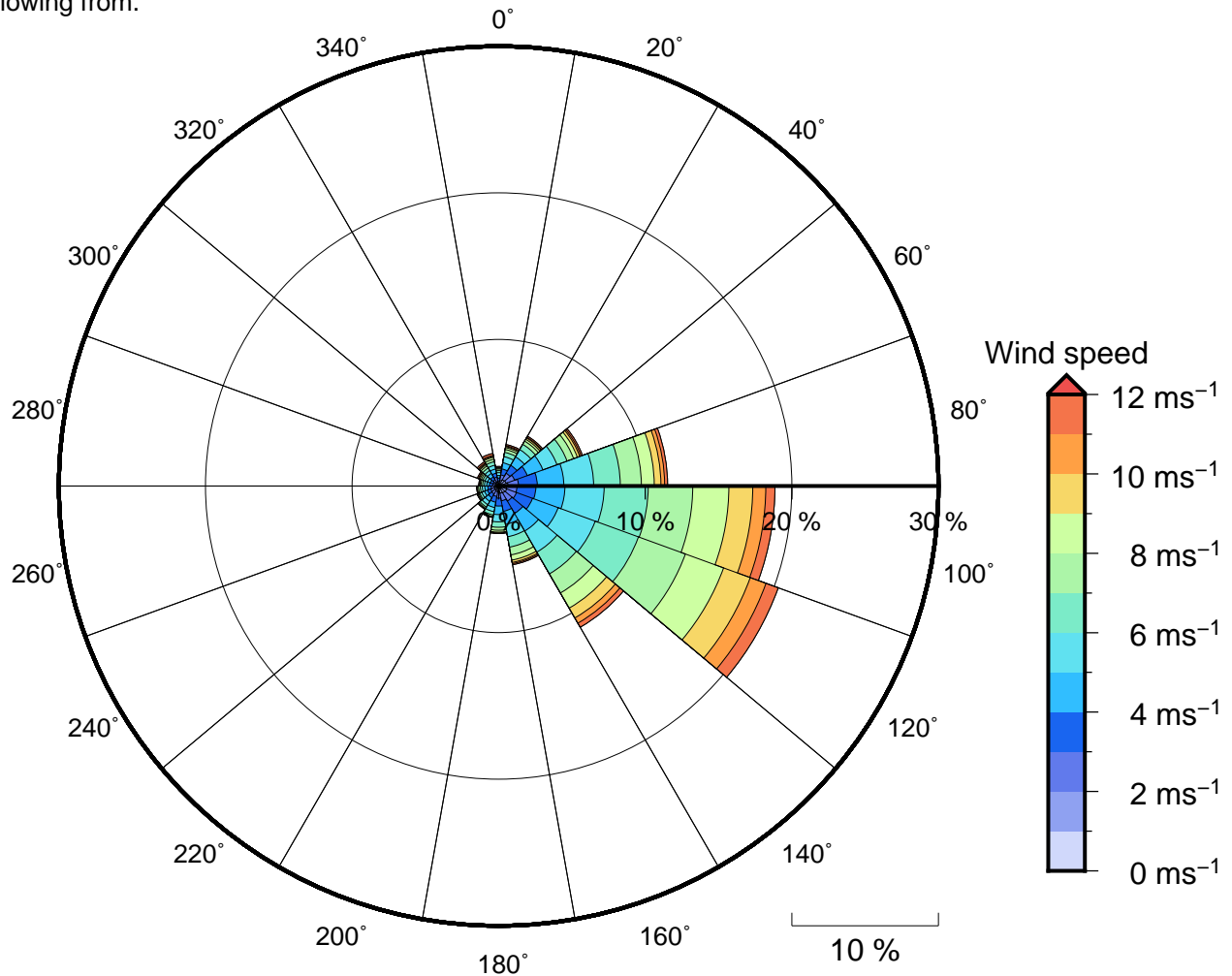
Figure 11 Annual wind rose for Nuku'alofa. Note that directions are where the wind is coming from.
