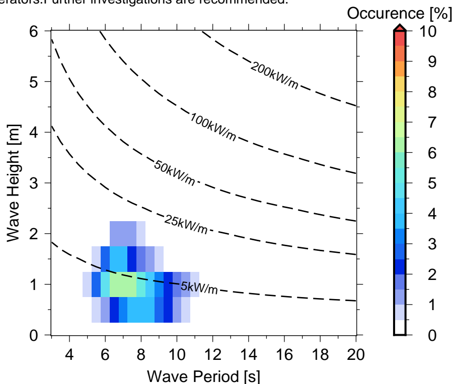
Figure 10 Occurrences of sea states in Nuku'alofa .
