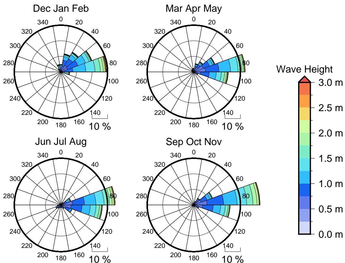
Figure 3 Seasonal wave roses for Nuku'alofa
