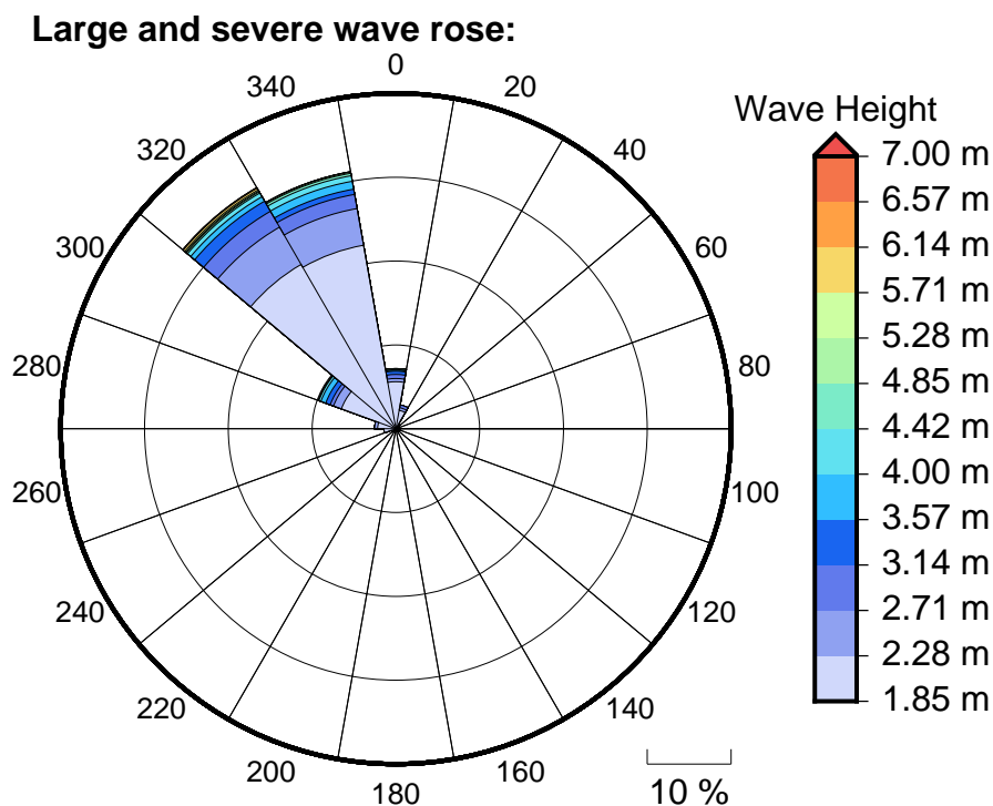
Figure 6 Large, severe and extreme wave roses for Pangai
