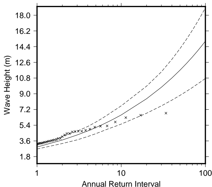
Figure 9 Extreme wave distribution for Pangai. The crosses represents the wave events that occurred since 1979. The plain line is the statistical distribution that best fit the past wave events. The dotted line show the upper and lower high confidence of the fit, there is a 95% chance that the fitted distribution lie between the two dashed lines.
