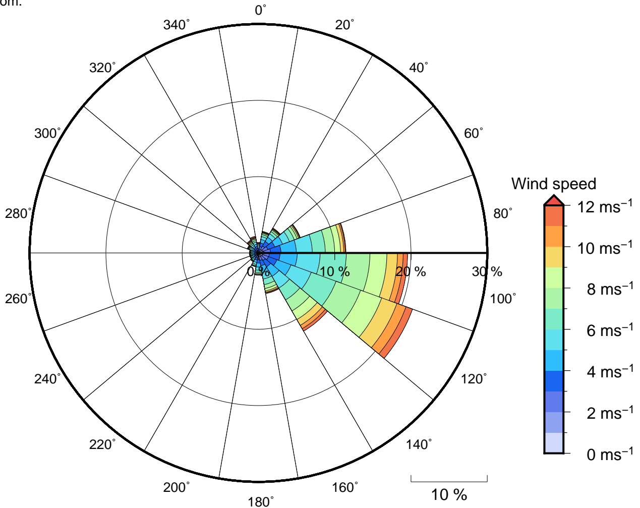
Figure 11 Annual wind rose for Pangai. Note that directions are where the wind is coming from.
