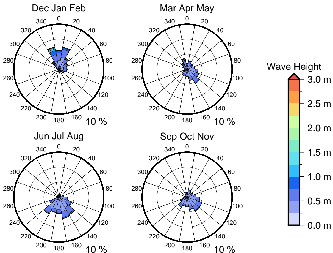
Figure 3 Seasonal wave roses for Pangai
