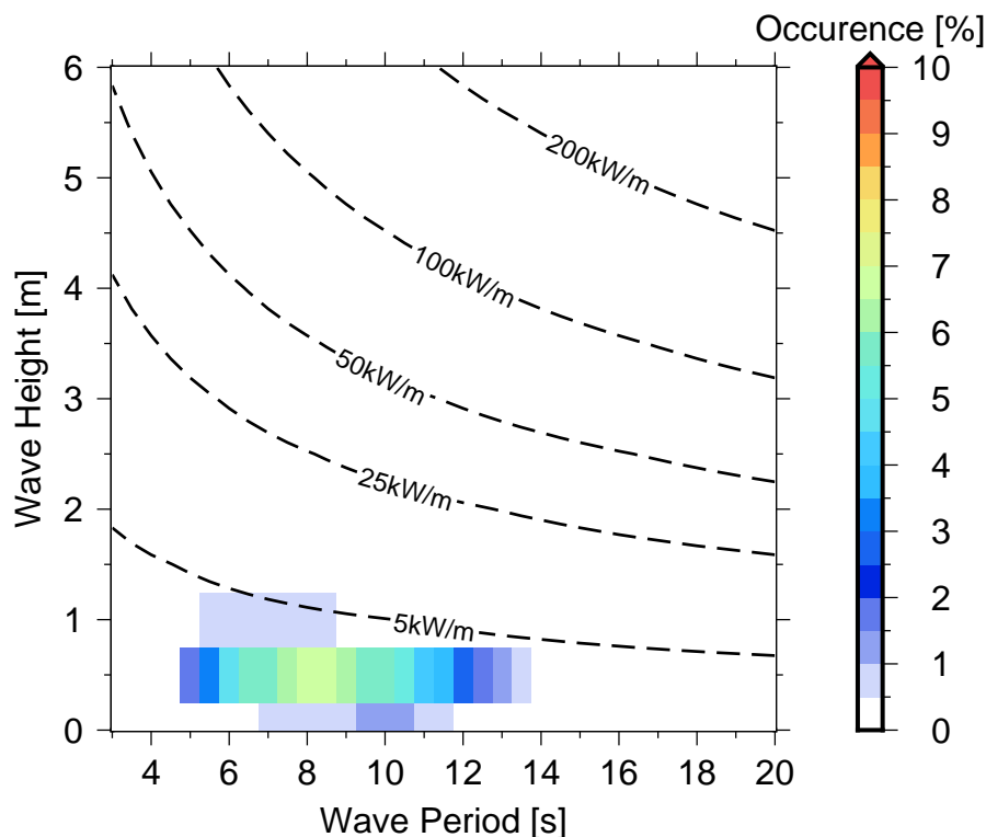
Figure 10 Occurrences of sea states in Pangai .
