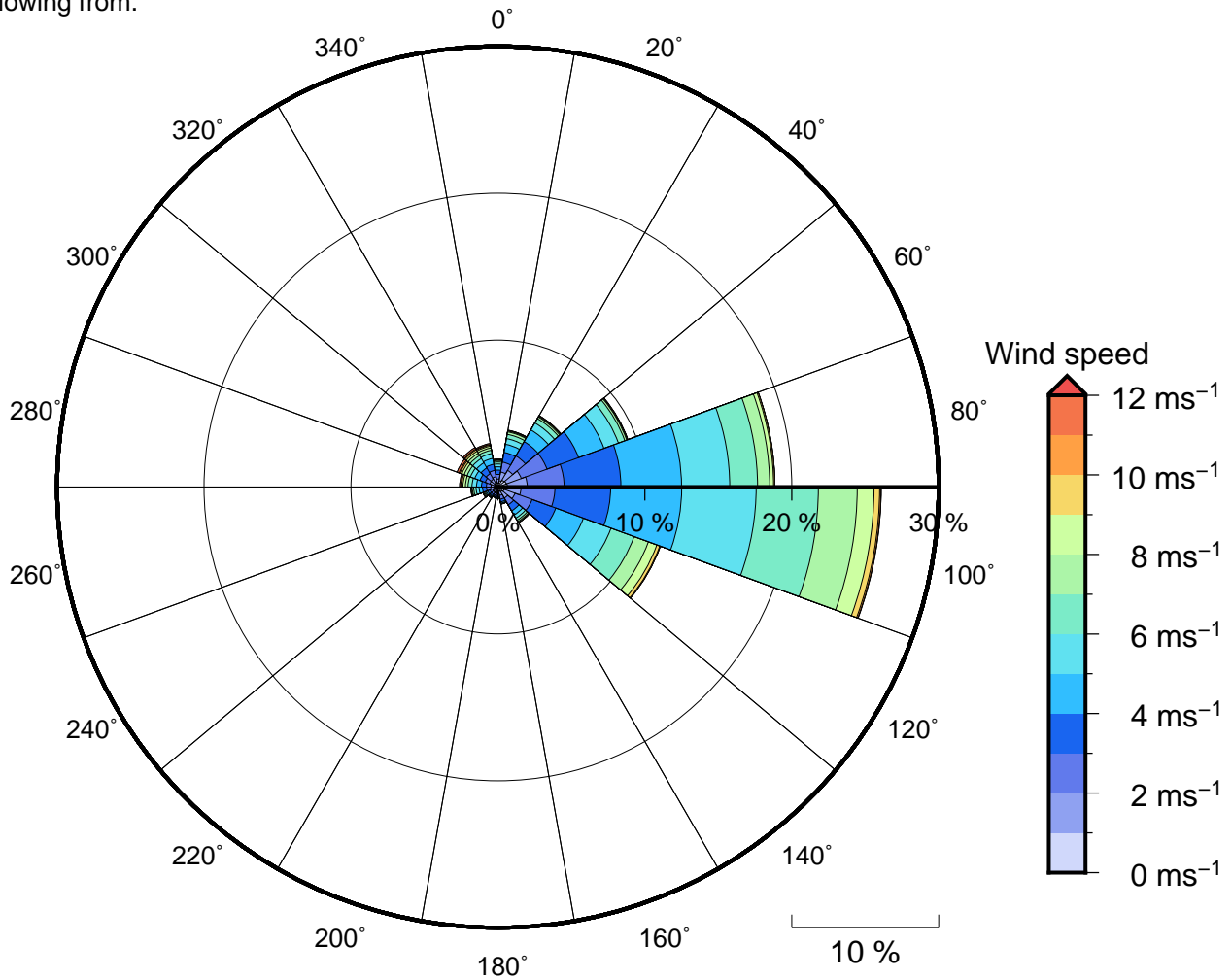
Figure 11 Annual wind rose for Fongafale. Note that directions are where the wind is coming from.
