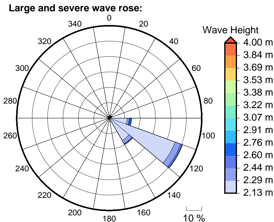
Figure 6 Large, severe and extreme wave roses for Fongafale
