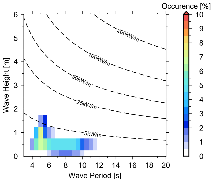
Figure 10 Occurrences of sea states in Luganville .
