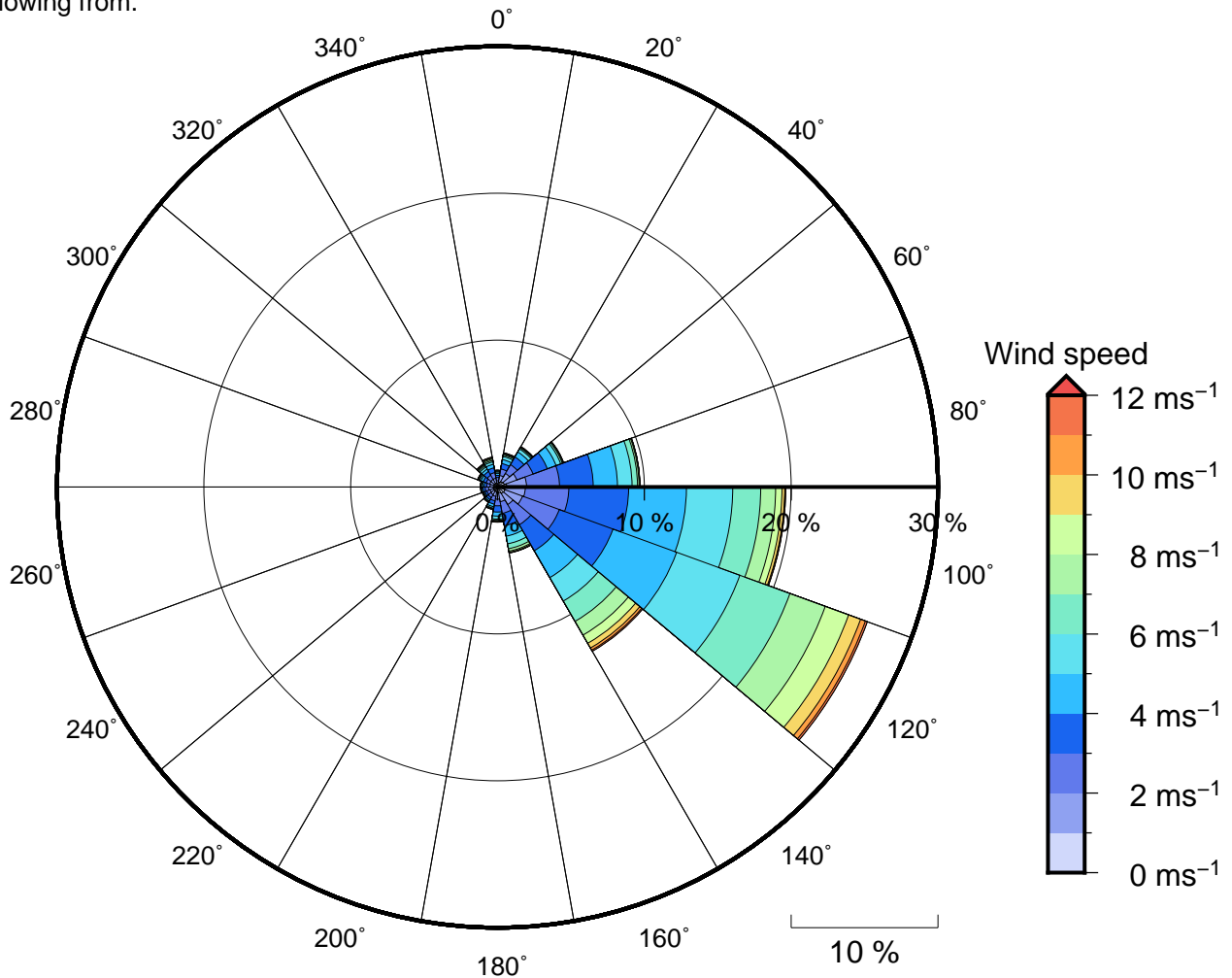
Figure 11 Annual wind rose for Luganville. Note that directions are where the wind is coming from .
