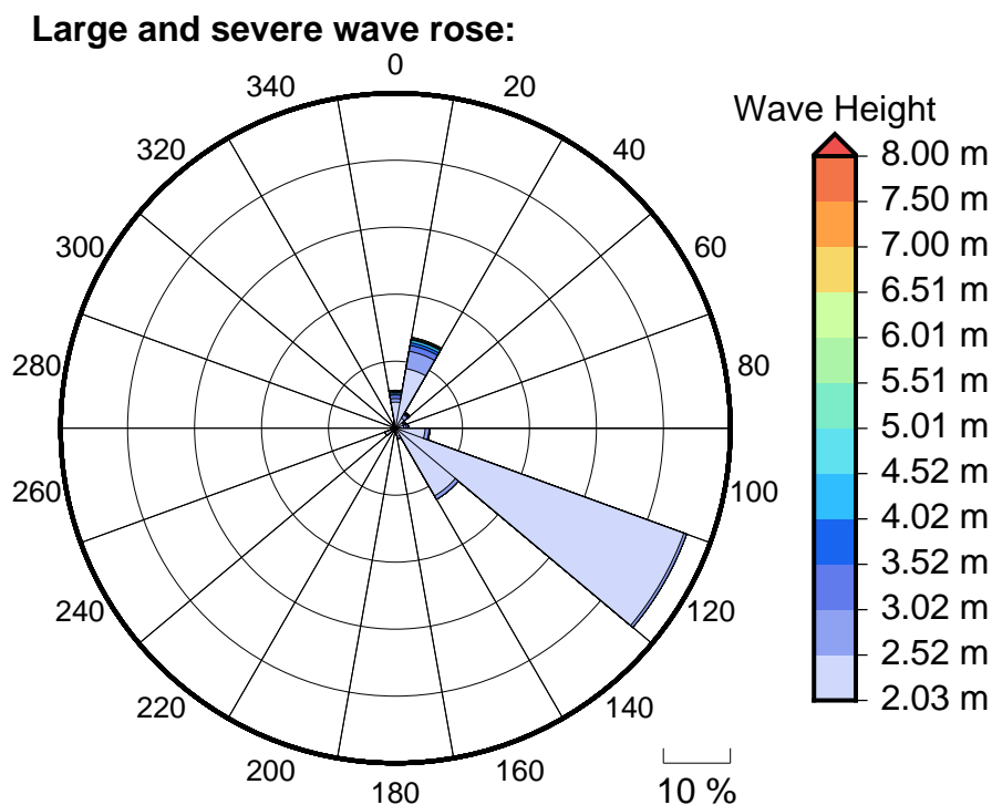
Figure 6 Large, severe and extreme wave roses for Luganville
