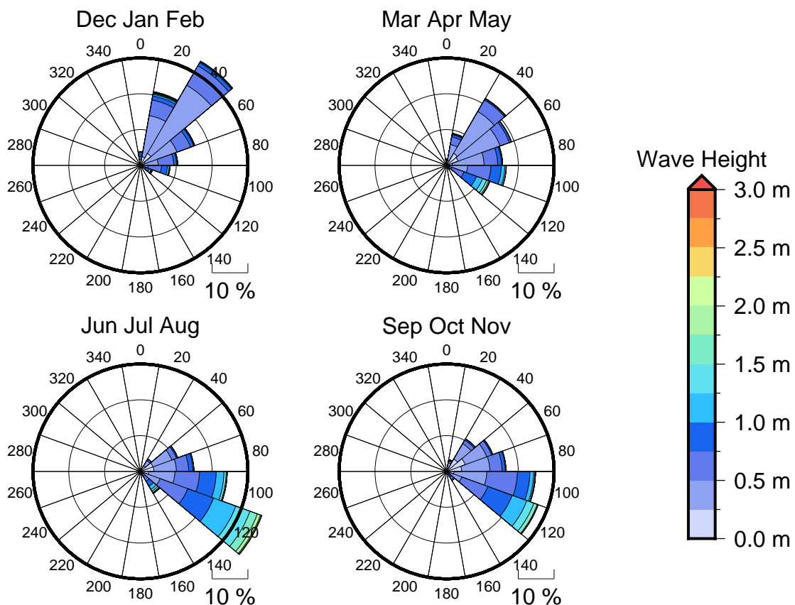
Figure 3 Seasonal wave roses for Luganville
