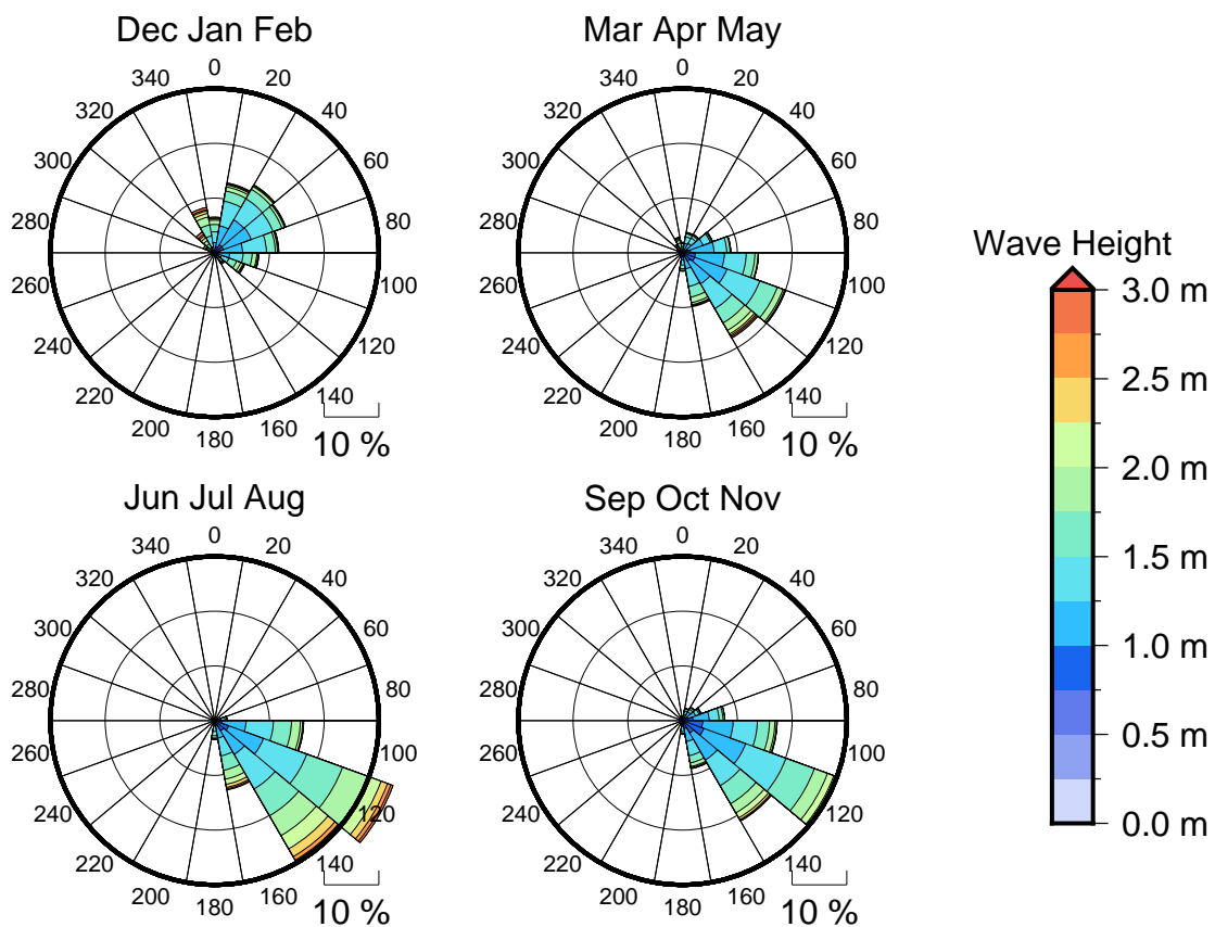
Figure 3 Seasonal wave roses for Honikulu Passage
