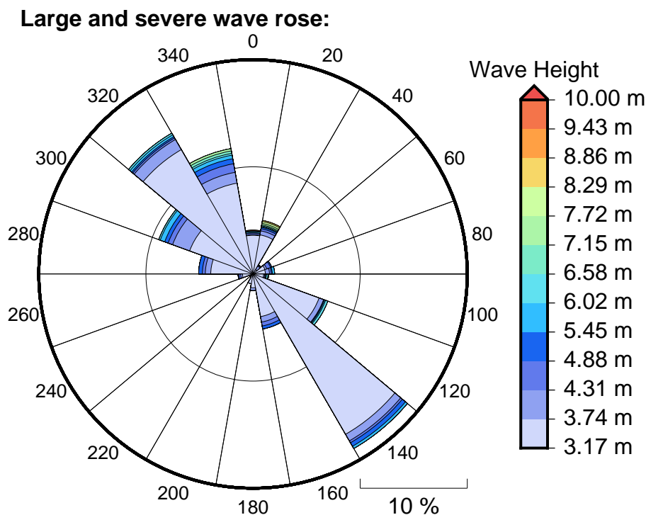
Figure 6 Large, severe and extreme wave roses for Honikulu Passage
