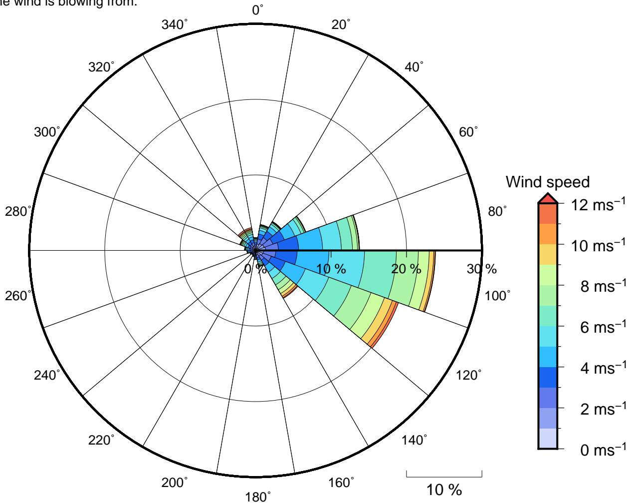
Figure 11 Annual wind rose for Honikulu Passage. Note that directions are where the wind is coming from.
