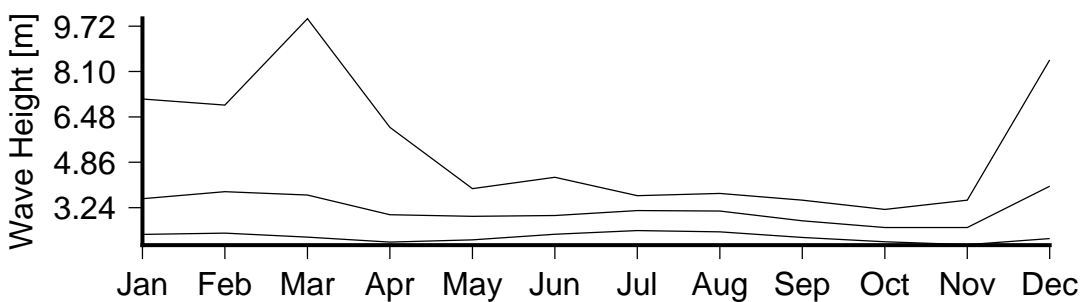
Figure 7 Monthly variation in large waves (90th percentile)(lower curve), severe waves (99th percentile) (middle curve) and the largest wave(upper curve) in Honikulu Passage.
