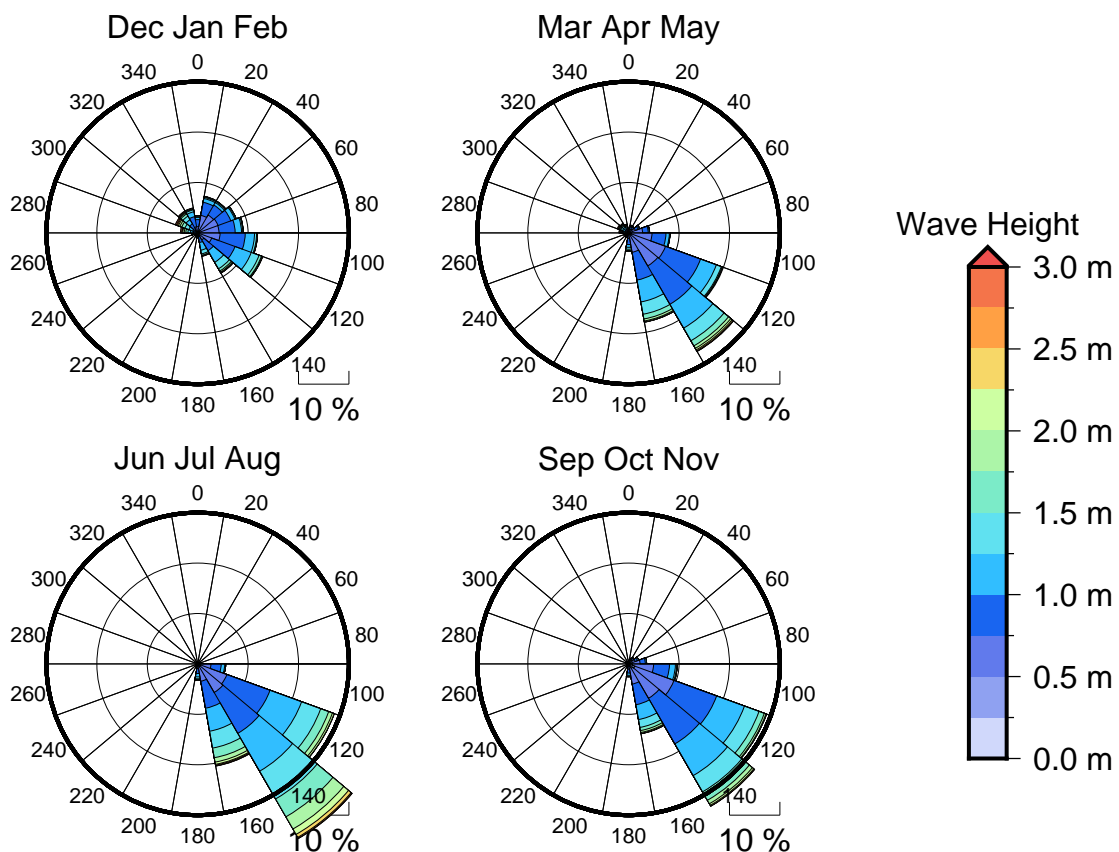
Figure 3 Seasonal wave roses for Leava
