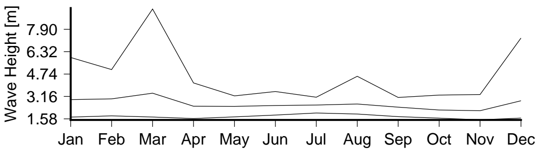
Figure 7 Monthly variation in large waves (90th percentile)(lower curve), severe waves (99th percentile) (middle curve) and the largest wave(upper curve) in Leava.
