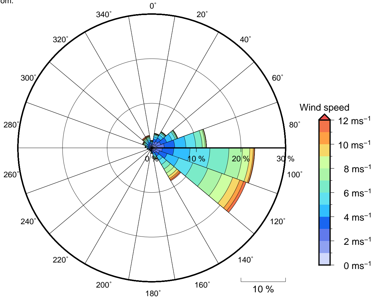
Figure 11 Annual wind rose for Leava. Note that directions are where the wind is coming from .
