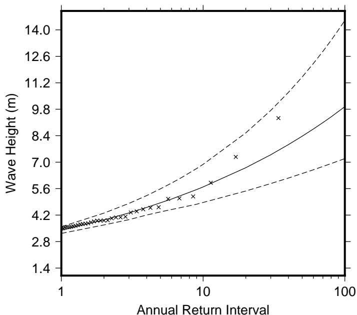
Figure 9 Extreme wave distribution for Leava. The crosses represents the wave events that occurred since 1979. The plain line is the statistical distribution that best fit the past wave events. The dotted line show the upper and lower high confidence of the fit, there is a 95% chance that the fitted distribution lie between the two dashed lines.
