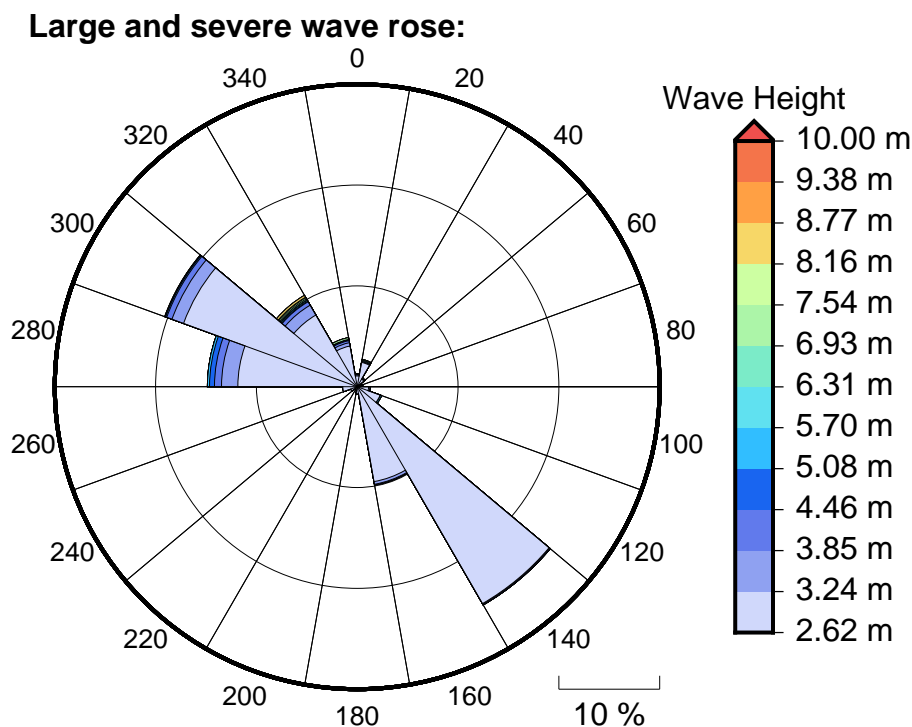
Figure 6 Large, severe and extreme wave roses for Leava
