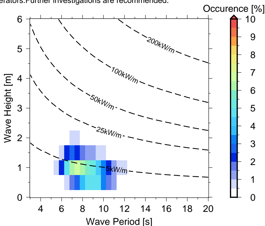
Figure 10 Occurrences of sea states in Leava .
