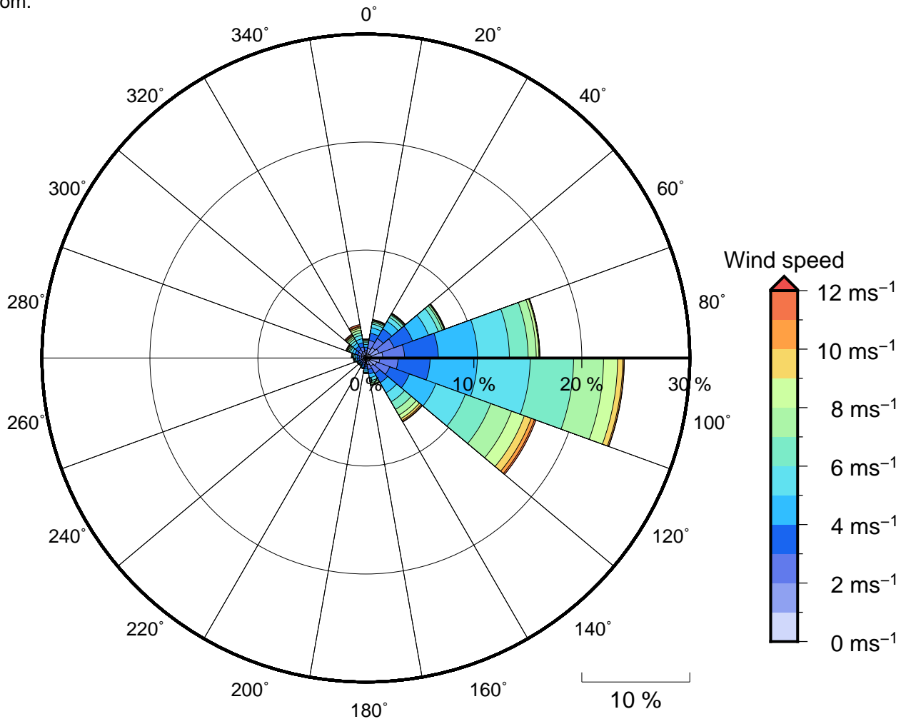
Figure 11 Annual wind rose for Apia. Note that directions are where the wind is coming from.
