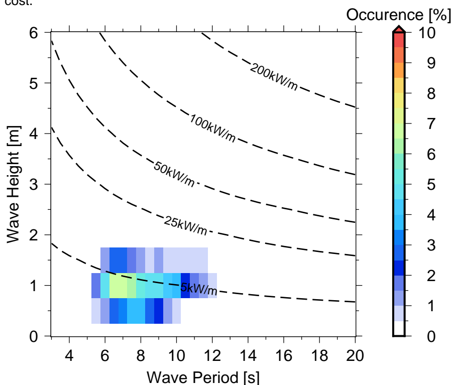
Figure 10 Occurrences of sea states in Apia .
