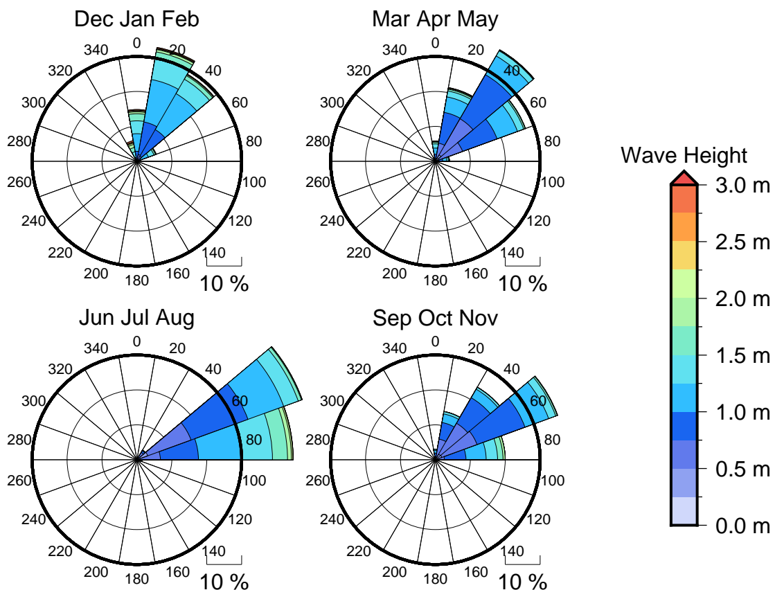
Figure 3 Seasonal wave roses for Apia
