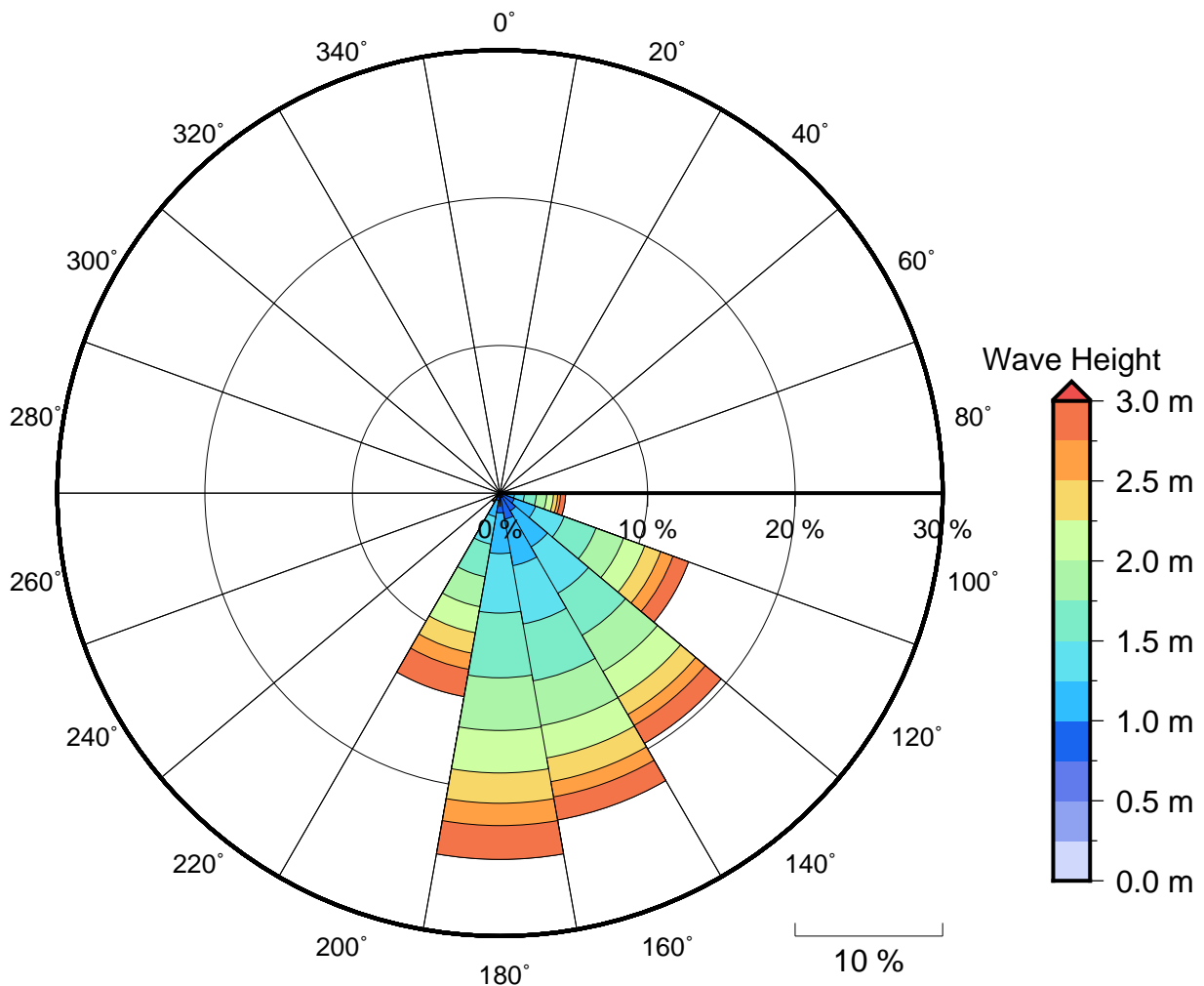
Figure 2 Annual wave rose for Wave Bouy location 1. Note that direction are where the wave are coming from.
