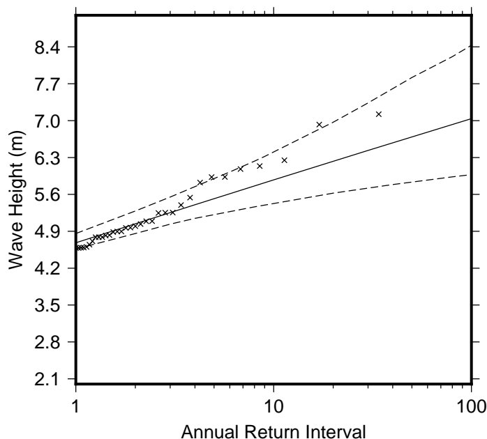
Figure 9 Extreme wave distribution for Wave Bouy location 1. The crosses represents the wave events that occurred since 1979. The plain line is the statistical distribution that best fit the past wave events. The dotted line show the upper and lower high confidence of the fit, there is a 95% chance that the fitted distribution lie between the two dashed lines.
