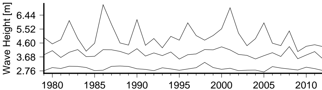
Figure 8 Annual variation in large waves (90th percentile)(lower curve), severe waves (99th percentile) (middle curve) and the largest wave(upper curve) in Wave Bouy location 1.
