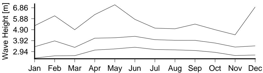
Figure 7 Monthly variation in large waves (90th percentile)(lower curve), severe waves (99th percentile) (middle curve) and the largest wave(upper curve) in Wave Bouy location 1.
