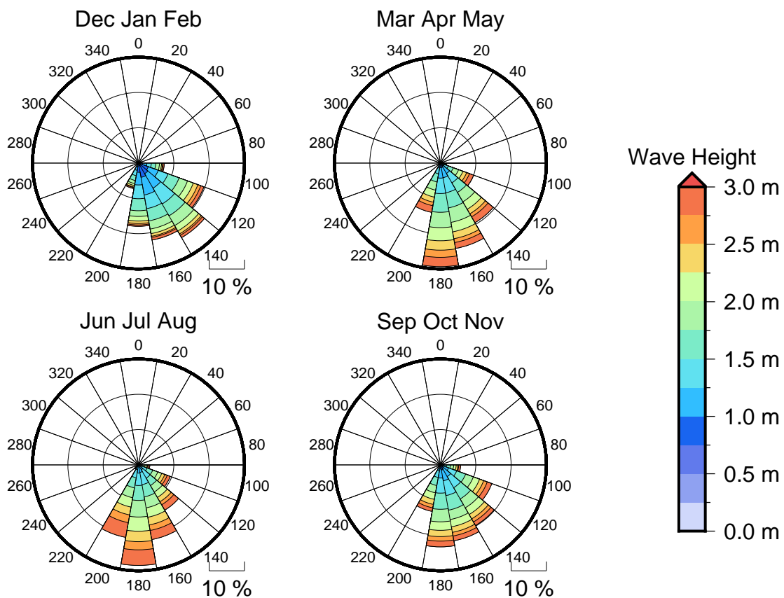
Figure 3 Seasonal wave roses for Wave Bouy location 1
