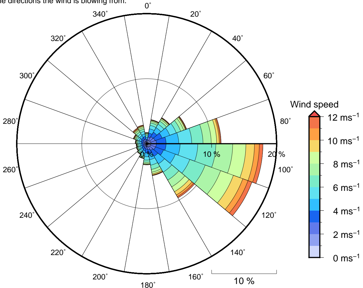
Figure 11 Annual wind rose for Wave Bouy location 1. Note that directions are where the wind is coming from.
