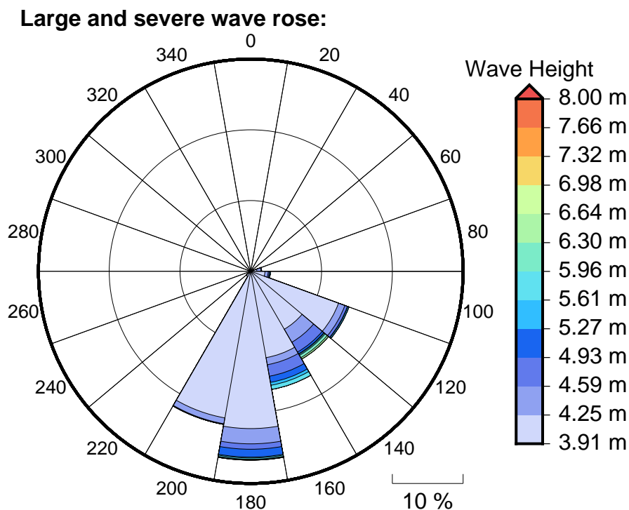
Figure 6 Large, severe and extreme wave roses for Wave Bouy location 1
