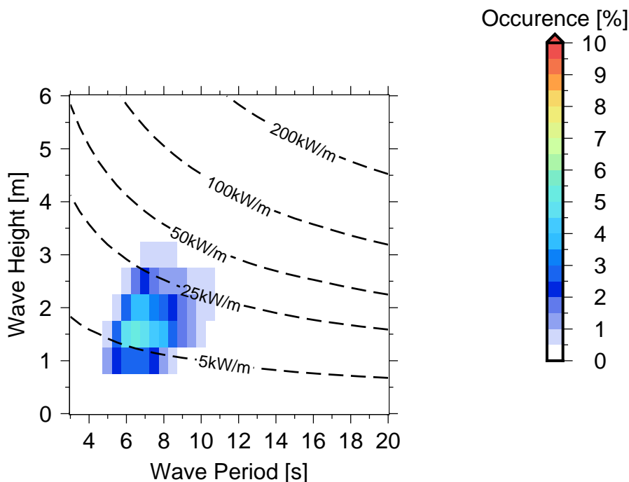
Figure 10 Occurences of sea states in Wave Bouy location 1 .
