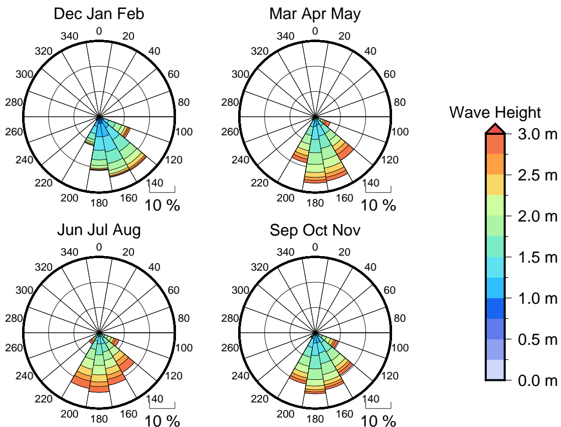
Figure 3 Seasonal wave roses for Kadavu
