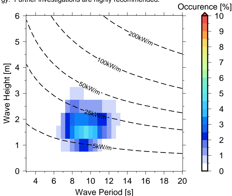
Figure 10 Occurrences of sea states in Kadavu .
