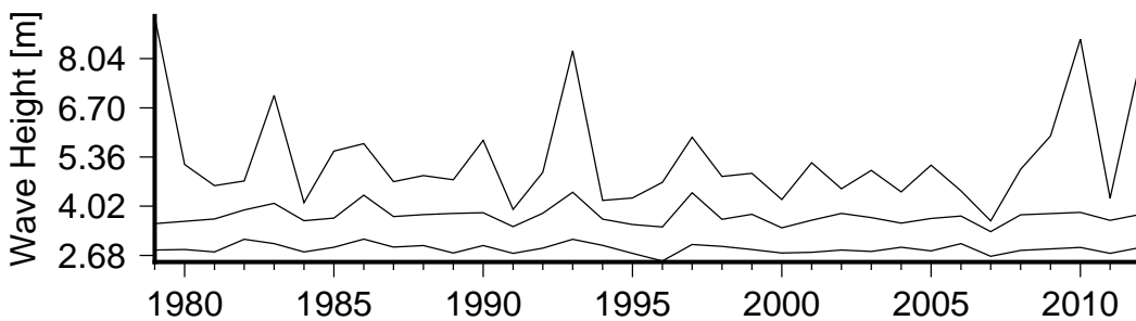
Figure 8 Annual variation in large waves (90th percentile)(lower curve), severe waves (99th percentile) (middle curve) and the largest wave(upper curve) in Kadavu.
