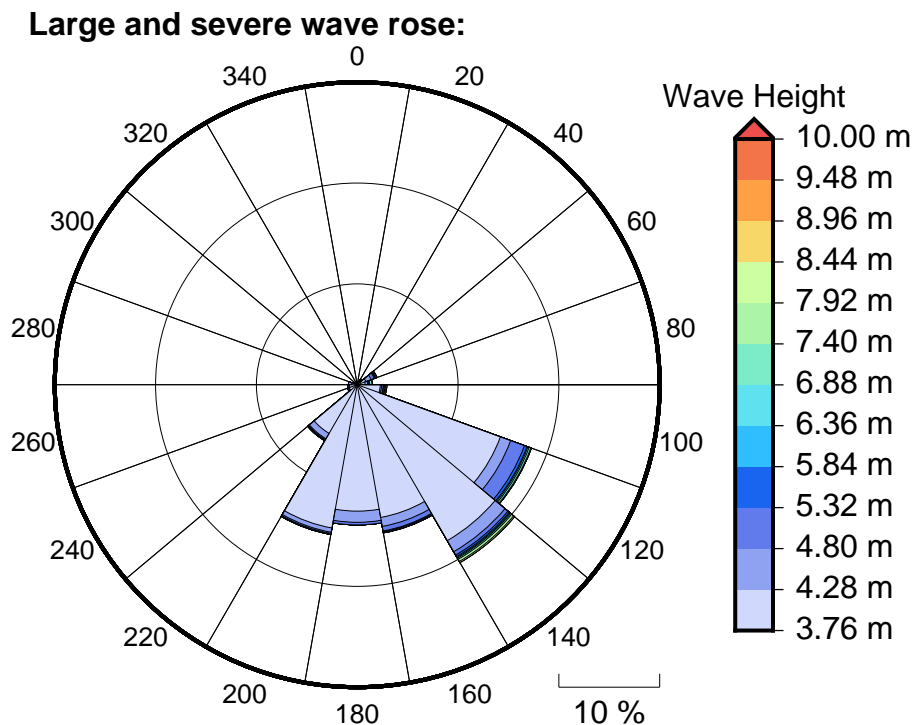
Figure 6 Large, severe and extreme wave roses for Kadavu
