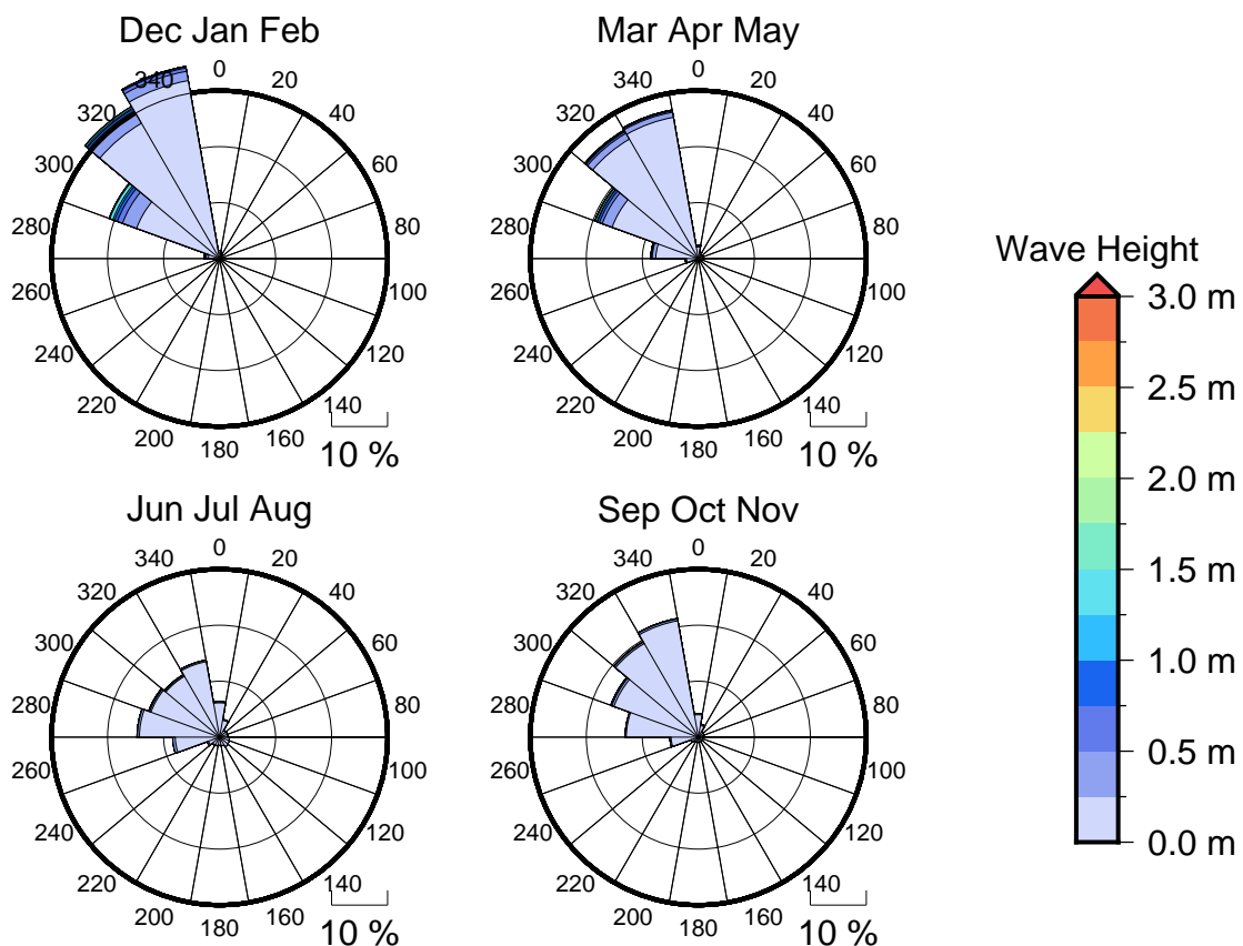
Figure 3 Seasonal wave roses for Lautoka
