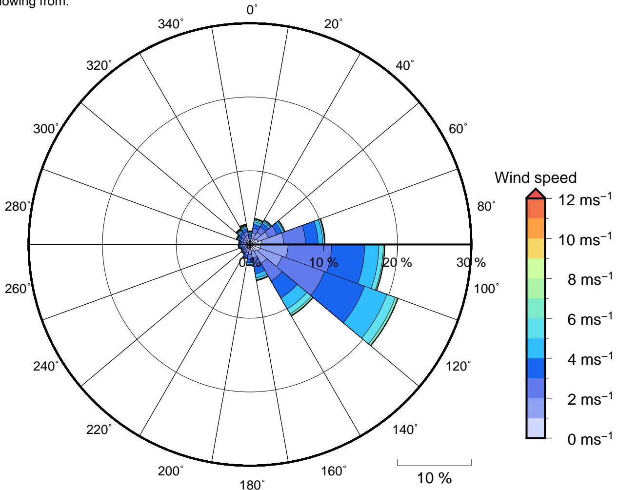
Figure 11 Annual wind rose for Lautoka. Note that directions are where the wind is coming from.
