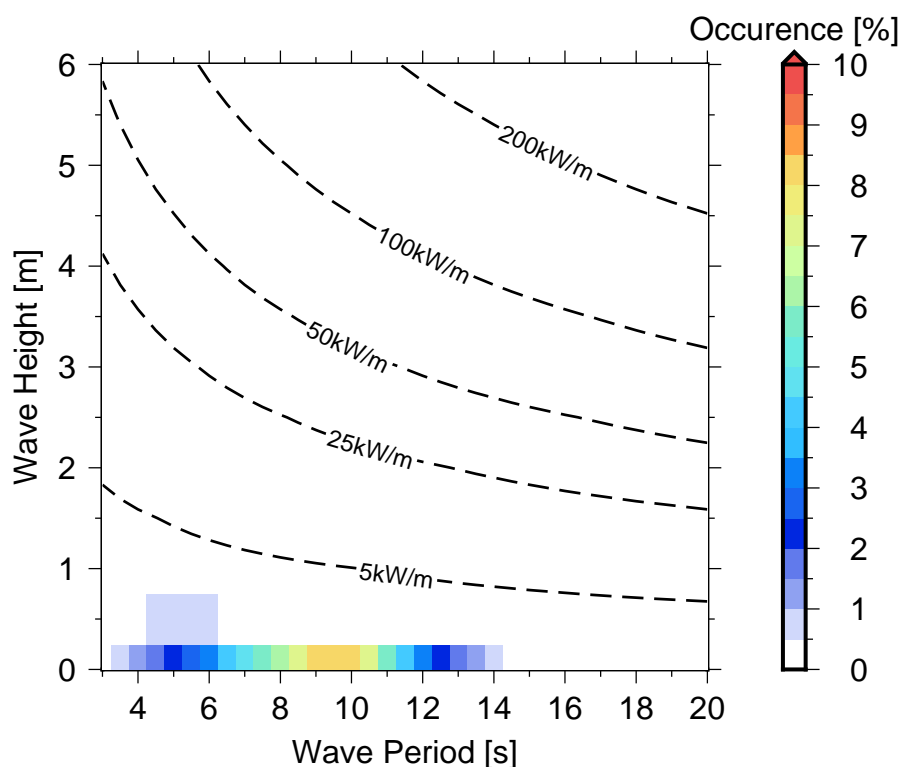
Figure 10 Occurrences of sea states in Lautoka .
