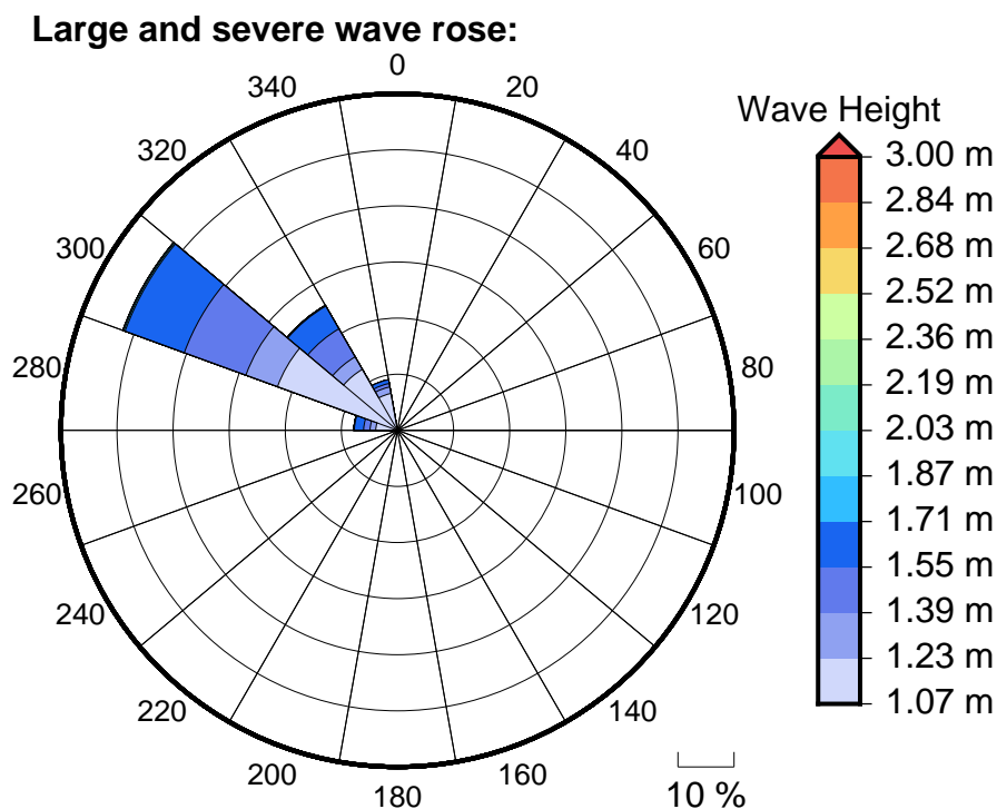
Figure 6 Large, severe and extreme wave roses for Lautoka
