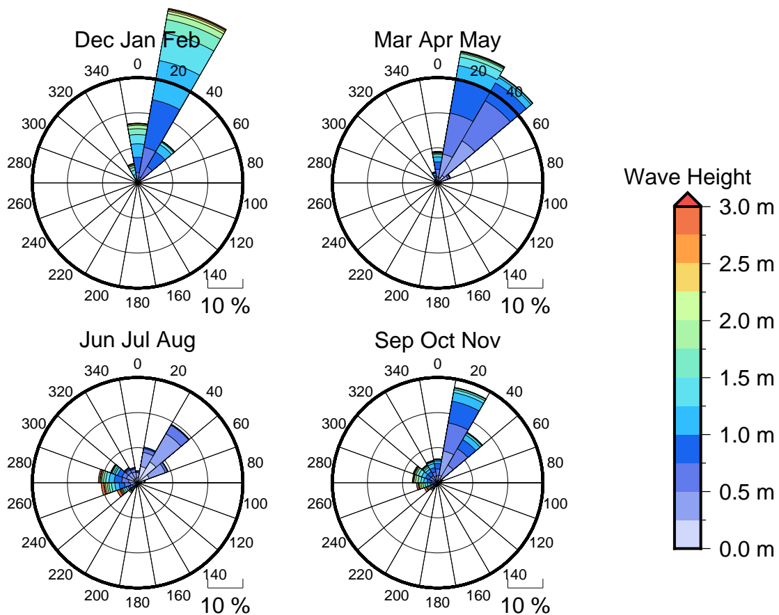
Figure 3 Seasonal wave roses for Guam
