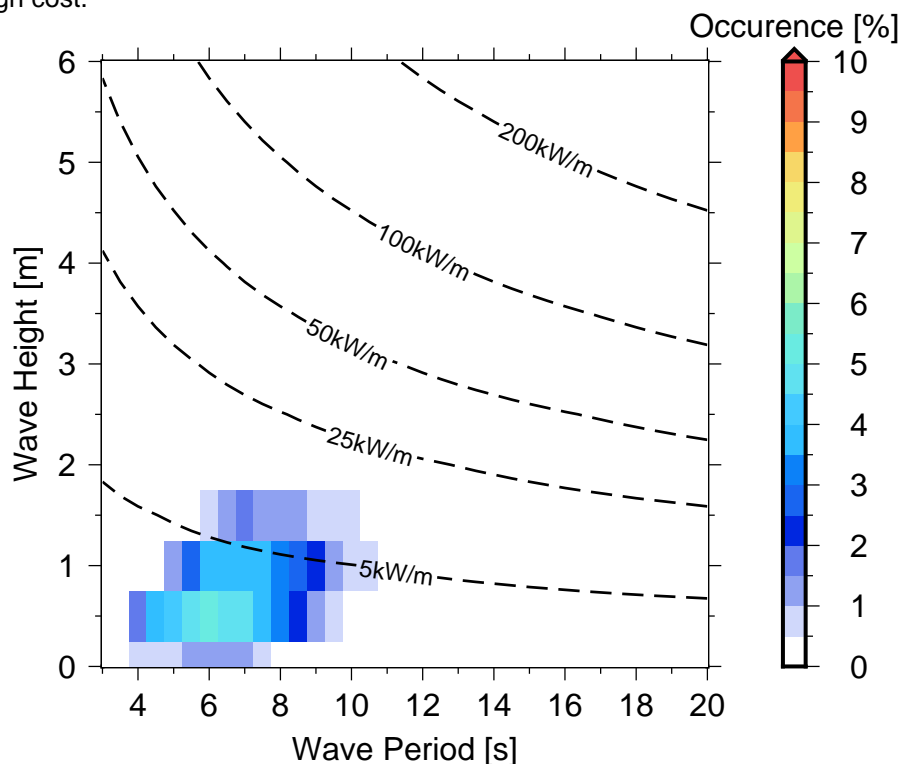
Figure 10 Occurrences of sea states in Guam .
