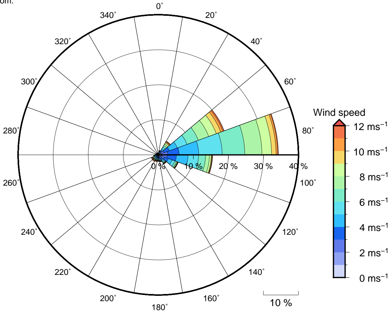
Figure 11 Annual wind rose for Guam. Note that directions are where the wind is coming from .
