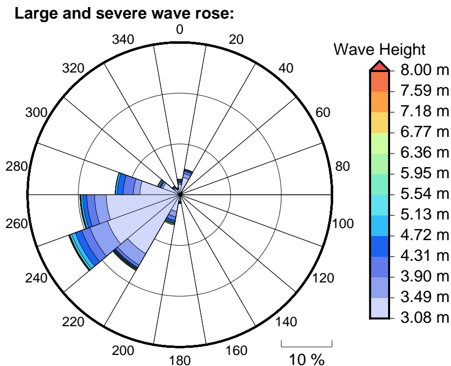
Figure 6 Large, severe and extreme wave roses for Guam
