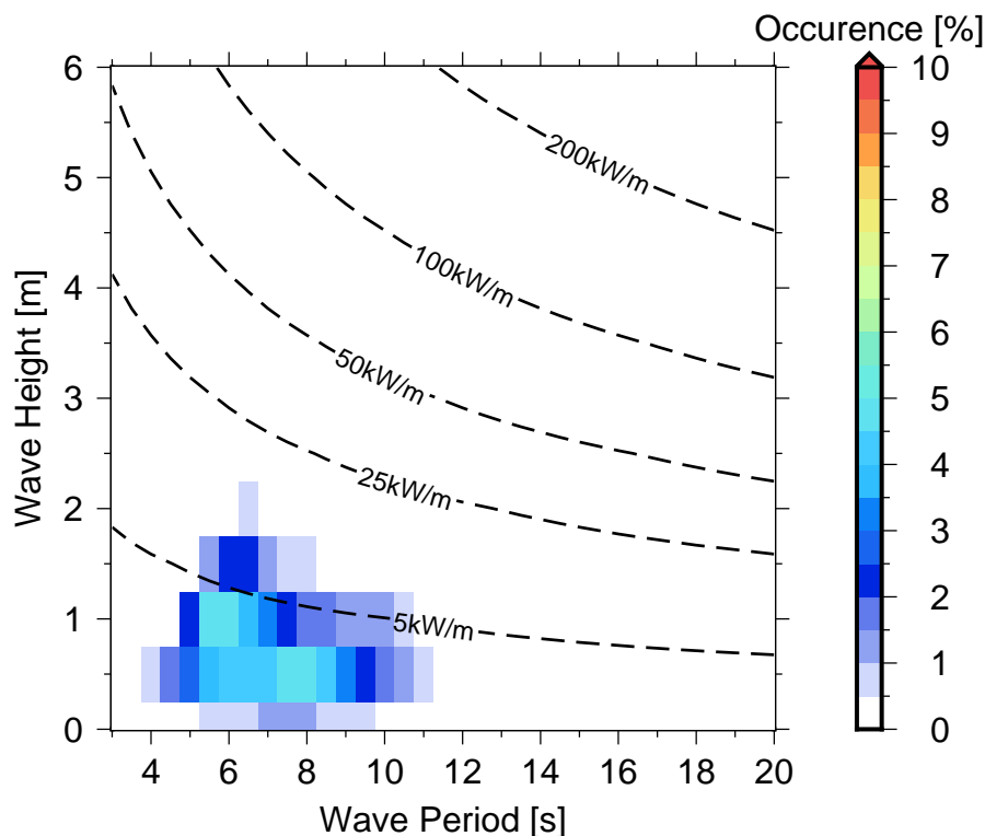
Figure 10 Occurrences of sea states in Kouaoua .
