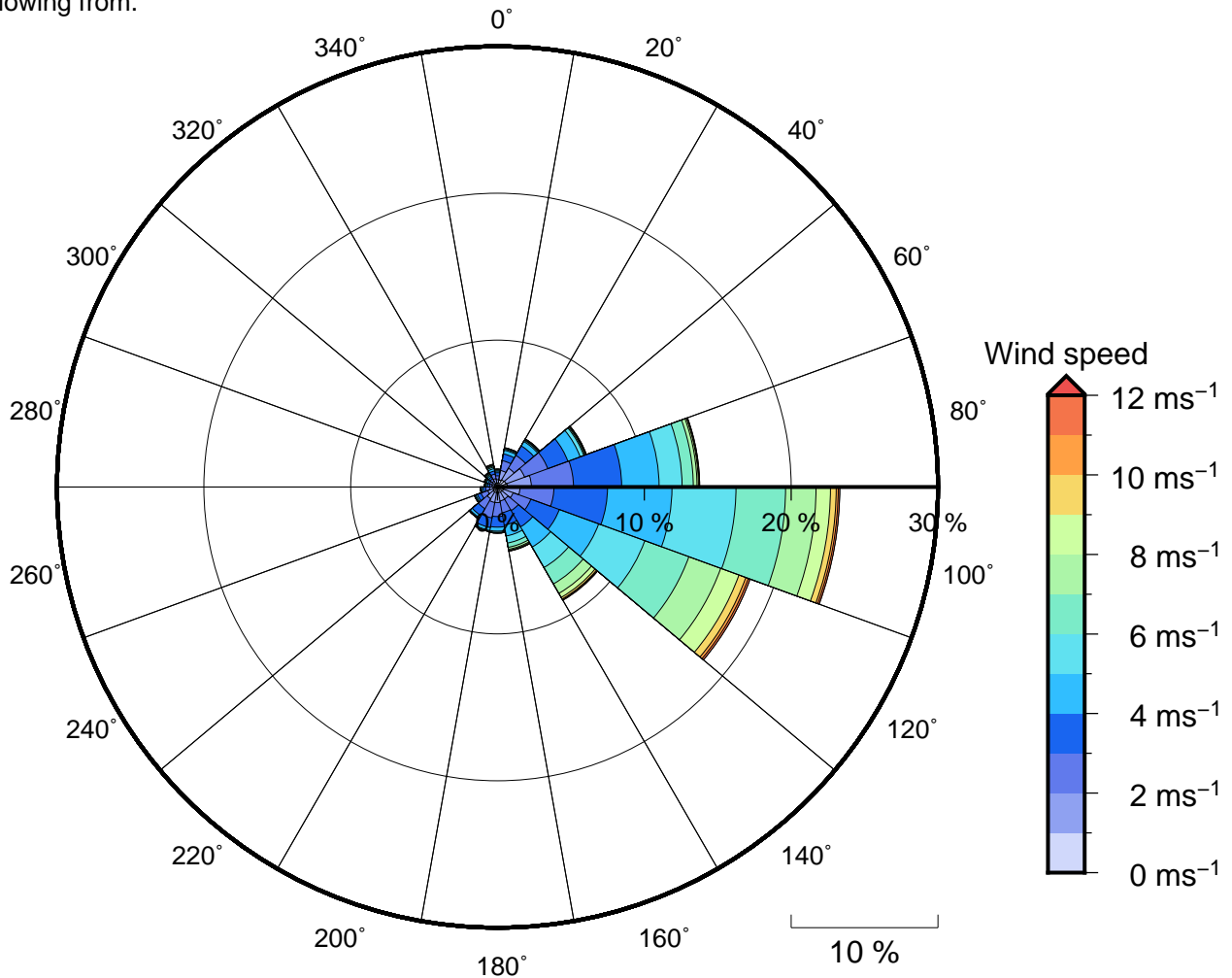
Figure 11 Annual wind rose for Kouaoua. Note that directions are where the wind is coming from .
