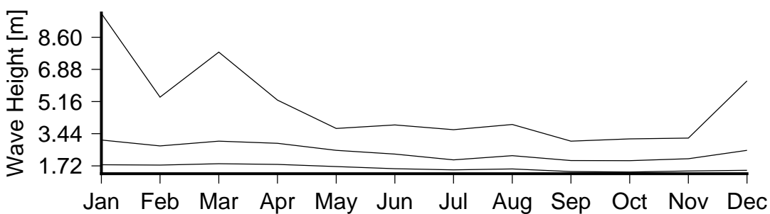
Figure 7 Monthly variation in large waves (90th percentile)(lower curve), severe waves (99th percentile) (middle curve) and the largest wave(upper curve) in Kouaoua.
