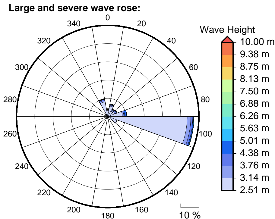
Figure 6 Large, severe and extreme wave roses for Kouaoua
