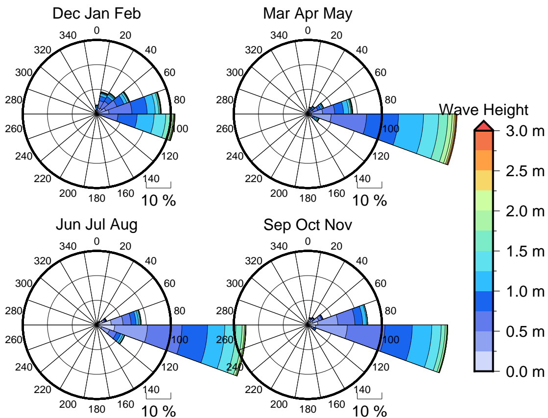
Figure 3 Seasonal wave roses for Kouaoua
