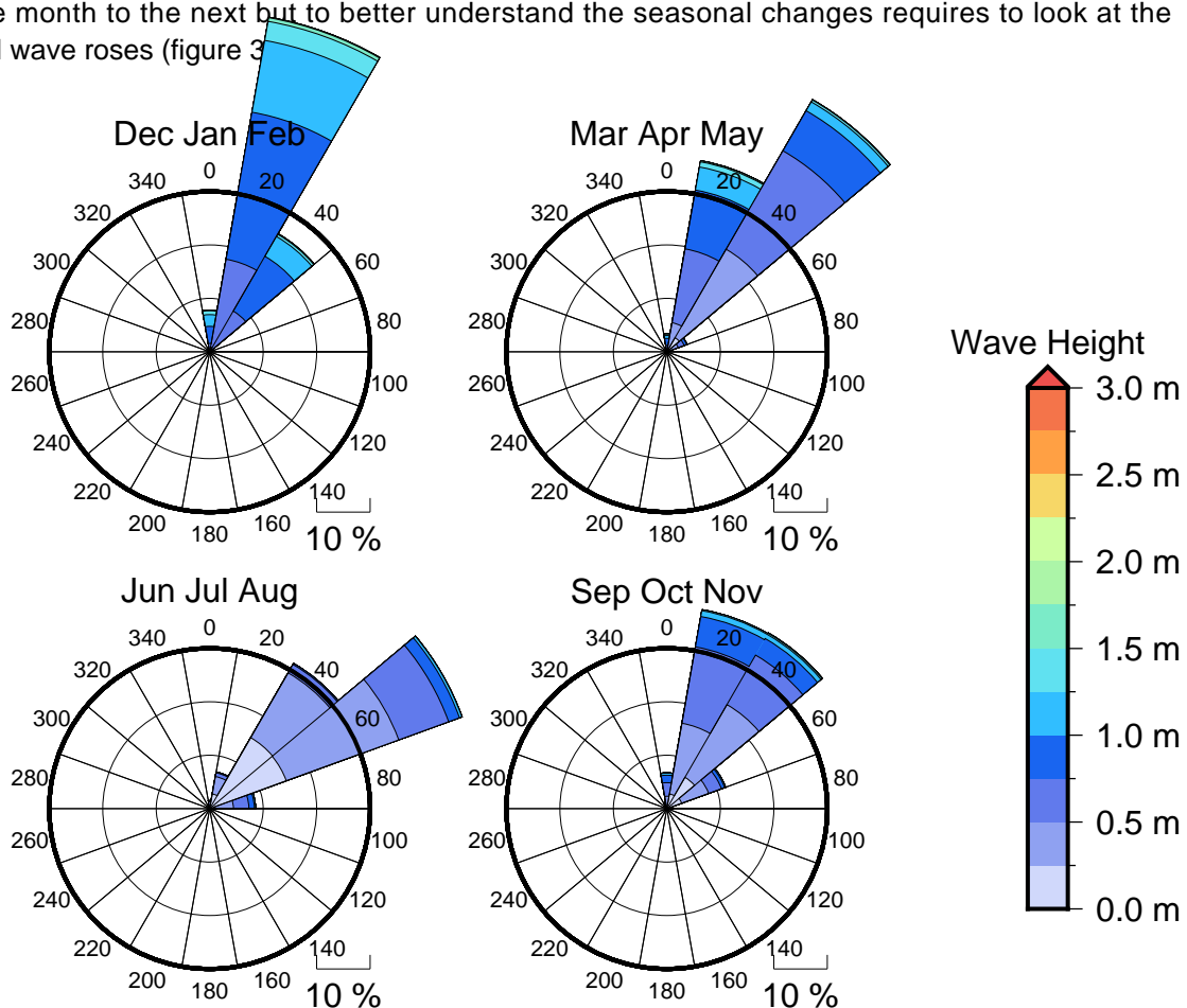
Figure 3 Seasonal wave roses for Vanimo
