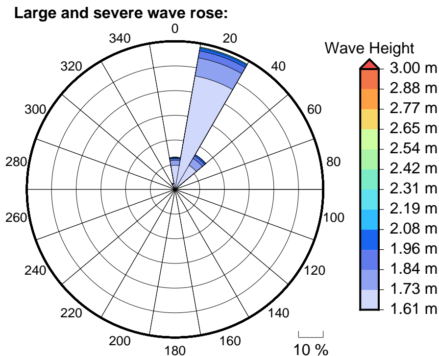
Figure 6 Large, severe and extreme wave roses for Vanimo
