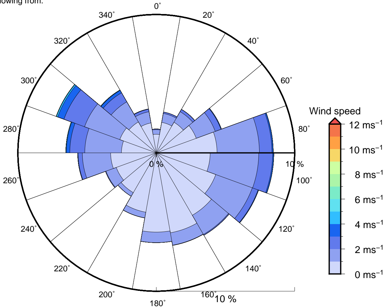
Figure 11 Annual wind rose for Vanimo. Note that directions are where the wind is coming from.
