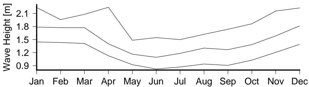
Figure 7 Monthly variation in large waves (90th percentile)(lower curve), severe waves (99th percentile) (middle curve) and the largest wave(upper curve) in Vanimo.
