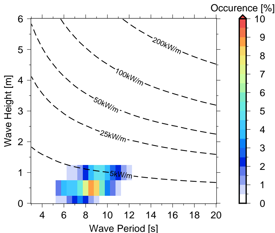
Figure 10 Occurrences of sea states in Vanimo .
