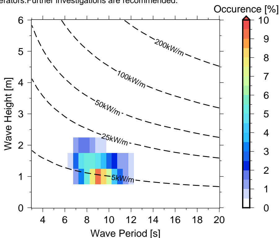
Figure 10 Occurrences of sea states in Nukunonu .
