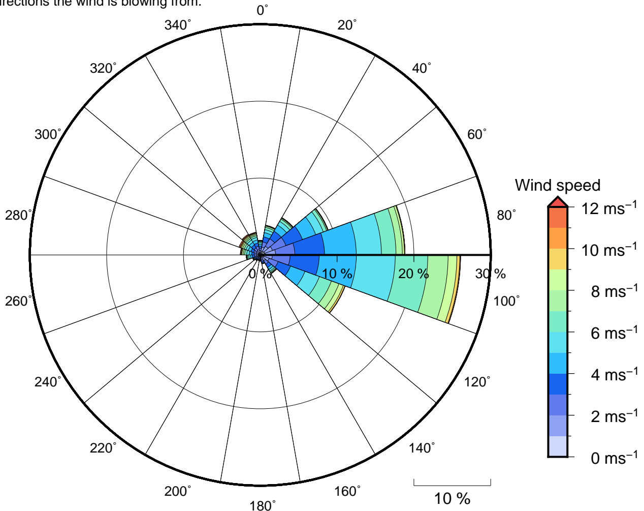
Figure 11 Annual wind rose for Funafuti Wave buoy. Note that directions are where the wind is coming from.
