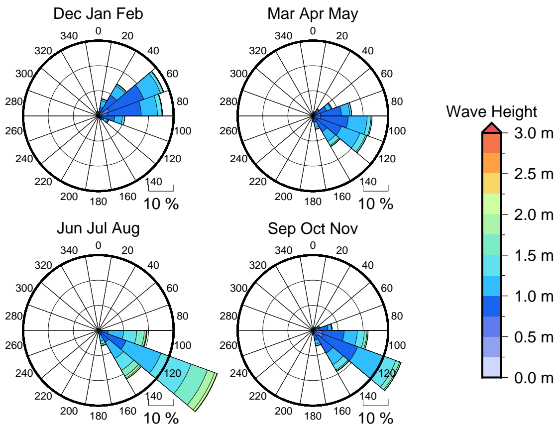
Figure 3 Seasonal wave roses for Funafuti Wave buoy
